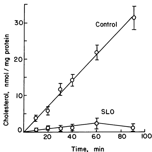
Figure 5. Conversion of [1,2- ^3 H]7-dehydrocholesterol to cholesterol by control ( n = 7 ) and Smith-Lemli-Opitz ( n = 4 ) liver microsomes. Mean \pm SD are plotted. Cholesterol was produced linearly over 90 min in the control incubations while little cholesterol was formed from 7-dehydrocholesterol by the Smith-Lemli-Opitz microsomes.
