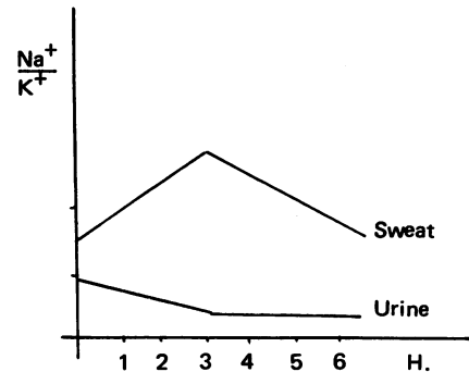
Fig. 4. Shows that \text{Na}^+/\text{K}^+ increases during the first part of walking (3h.) and then decreases. In the urines \text{Na}^+/\text{K}^+ decreases during 6h.
