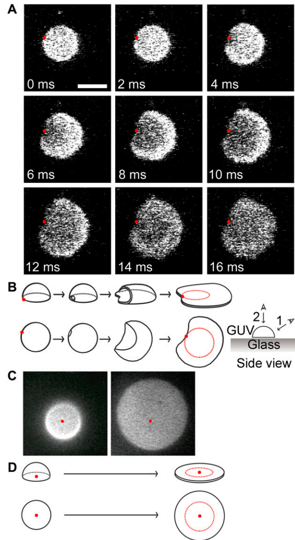
FIGURE 2 Rupture mechanisms for isolated GUVs. For all images, the focal plane was the glass surface. Scale bar in A , 5 \mu\text{m} ; same scale for all images. ( A ) The major isolated rupture pathway. This image sequence, collected at 500 fps, shows that the changes in the geometry of the fluorescence pattern and in the average fluorescence intensity per unit area are consistent with the rupture of a single glass-adsorbed GUV. The red dots are in identical locations in each image and demonstrate that the observed fluorescence emission patterns have a common edge point. This edge point appears to be at or near the point at which rupture was initiated. A movie is available online in Supplementary Material (Fig2A.mov). ( B ) Schematic illustration of the rupture process shown in A . Two viewpoints are shown: ( upper ) viewpoint 1 is from the side of the vesicle, but looking down upon the surface; ( lower ) viewpoint 2 is from above the vesicle. Red dots have the same meaning as in A . The red circle on the final planar bilayer patch identifies the boundary of the surface-adsorbed lipid structure before rupture. ( C ) The minor isolated rupture pathway. A glass-adsorbed GUV ( left ) formed a planar bilayer patch ( right ) that was circular, with approximately the same center as the original adsorbed lipid structure. The location of the center of the circular fluorescence distribution in the left image is identified in both images by the red dot. Integration time, 64 ms. Time between images, ~8 ms. ( D ) Schematic illustration of the rupture process shown in C . As in B , two viewpoints are shown. The red circles and red dots have the same meanings as in B and C , respectively.
