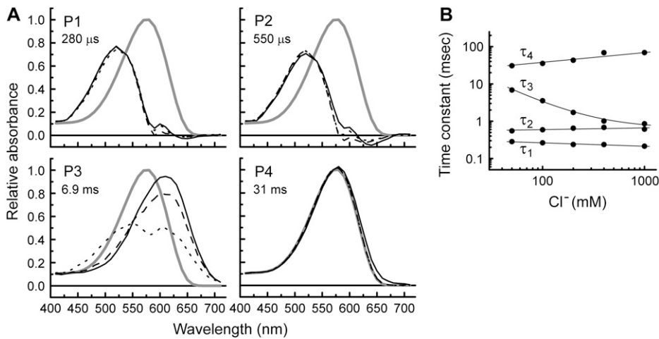
FIGURE 7 Results of the global fitting of the flash-photolysis data of wild-type pHR. (A) Absorption spectra of unphoto-lyzed (ground) state ( P_0 ) and four kinetically distinguishable intermediates at three representative \text{Cl}^- concentrations (solid line, 50mM; dashed line, 400 mM; dotted line, 1000 mM). The P_3 state shows the largest dependence on \text{Cl}^- concentration, both in terms of the time constant ( \tau_3 ) and the absorption spectrum. The figures represent the time constants corresponding to the states in 50 mM NaCl, pH 7.0, at 20°C. (B) Time constants for the photochemical transitions as a function of \text{Cl}^- concentration.
