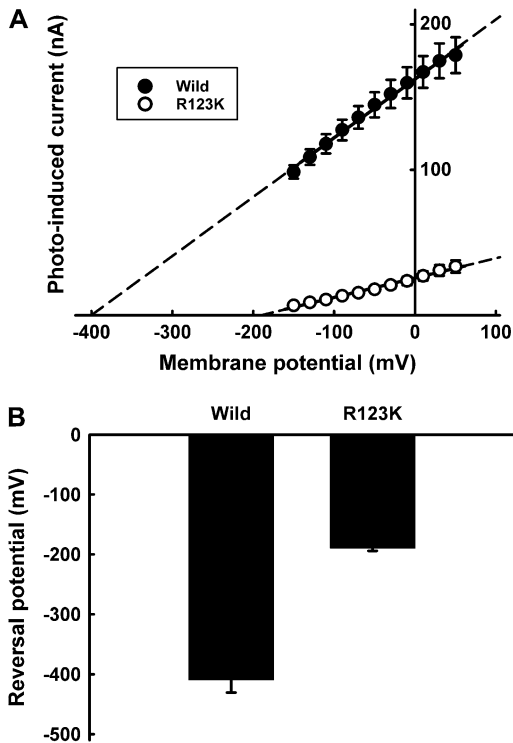
FIGURE 4 Reversal potentials for wild-type and mutant (R123K) pHRs. (A) Representative I-V curve at steady state for wild-type and mutant (R123K) pHRs. The concentration of \text{Cl}^- in the perfusion medium (as NaCl) was 100 mM. (B) Reversal potentials for wild-type and mutant (R123K) pHRs. The values were determined from the x -intercepts by the extrapolation of the lines describing the I-V relationship. Data represent mean \pm SE ( n = 6 ).
