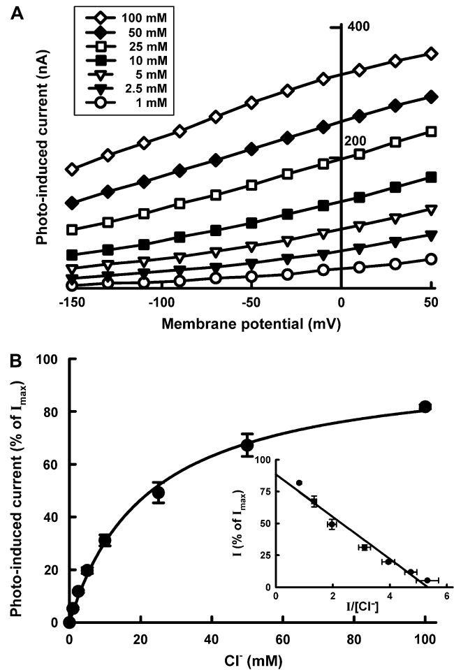
FIGURE 5 Saturation kinetics of the photoinduced \text{Cl}^- pump activity of pHR. (A) Representative I-V curve at steady state in pHR-expressing oocytes at increasing concentrations of \text{Cl}^- (as NaCl) (1–100 mM). (B) Photoinduced currents at -50 mV indicative of \text{Cl}^- entry as a function of \text{Cl}^- concentration. The experiment was repeated five times with different oocytes. Since the expression levels of pHR varied among the oocytes, data were normalized by the value of I_{\text{max}} , calculated using Eq. 1, in each oocyte. The inset shows the Eadie-Hofstee plot. The K_{0.5} and I_{\text{max}} values calculated with a Michaelis-Menten-type equation (Eq. 1) were 24.0 \pm 2.5 mM and 324 \pm 22 nA, respectively. Data represent the mean \pm SE ( n = 5 ).
