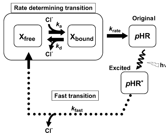
FIGURE 9 A kinetic model for the photoinduced current at steady state for p\text{HR} on the basis of the photocycle. Under conditions of continuous illumination, all intermediates attain steady state, the excited p\text{HR} consists almost entirely of the population of intermediate molecules in the rate-determining transition, and the photoinduced current is governed mainly by the rate determining process. Therefore, focusing only on the intermediates involved in the photoinduced current at steady state, we simplify the photocycle scheme of p\text{HR} and construct the kinetic model describing the photoinduced current due to \text{Cl}^- transport via p\text{HR} . The kinetic model is comprised of two processes: one is the fast transition of intermediates corresponding to \text{Cl}^- translocating and releasing processes, and the other is the rate-determining transition corresponding to \text{Cl}^- binding processes. According to the mass conservation, a mass-balance equation consists of the original p\text{HR} , the photoexcited p\text{HR} ( p\text{HR}^* ) molecules, and \text{Cl}^- free and bound intermediates ( X_{\text{free}} and X_{\text{bound}} , respectively). Taking into consideration that the k_{\text{rate}} value is much smaller than any other rate constants ( k_{\text{fast}} , k_a , and k_d ), the photoinduced current at steady state is reduced to Eq. 3.
