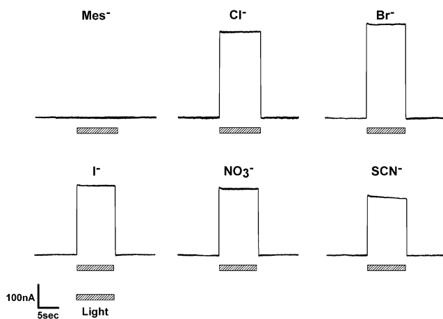
FIGURE 1 Traces of representative currents photoinduced via pHR expressed heterologously in pHR-expressing Xenopus oocytes were superfused with standard buffer containing different anions (as sodium salts) at a concentration of 100 mM. The hatched bars below the current traces indicate the period (10 s) of illumination with green light ( 530 \pm 18 nm). In control oocytes with no pHR expression, there were no detectable currents in response to light pulses (data not shown).
