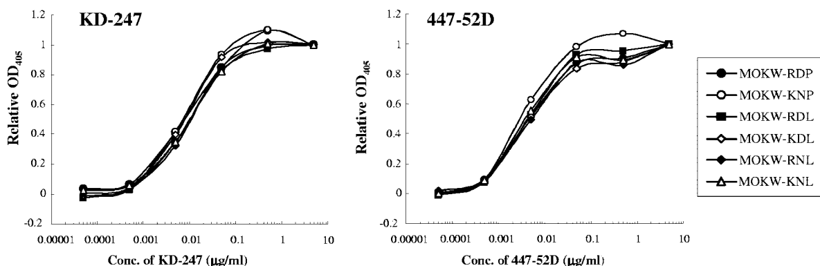
FIG. 7. Binding affinity of anti-V3 MABs to monomeric gp120. Viral lysates for each MOKW pseudovirus were used. gp120 was captured onto microtiter wells using a sheep polyclonal antibody specific for the C terminus of gp120. Serial dilutions of KD-247 or 447-52D were tested for binding by ELISA. Because of differences in the amount of bound gp120, optical density at 405 nm (OD 405 ) values were normalized to saturating levels of antibody (5 μg/ml) for comparison. Conc, concentration.
