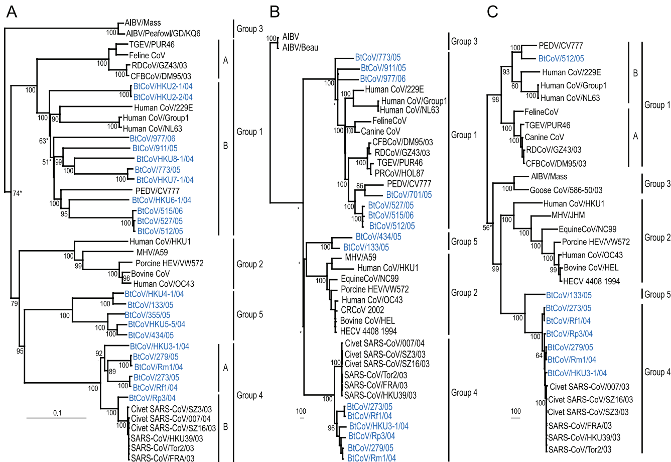
FIG. 1. Phylogenetic relationships of helicase (A), spike (B), and nucleocapsid (C) genes based on alignments of 1,797, 2,204, and 1,812 nucleotides, respectively. Breda virus (AY427798) was used to root the trees. Numbers at branch nodes indicate neighbor-joining bootstrap values of \geq 50\% . Nodes with Bayesian posterior probabilities of \leq 95\% are indicated with asterisks. Bar, 0.1 nucleotide substitution per site (A) or 100 nucleotide substitutions per site (B and C).
