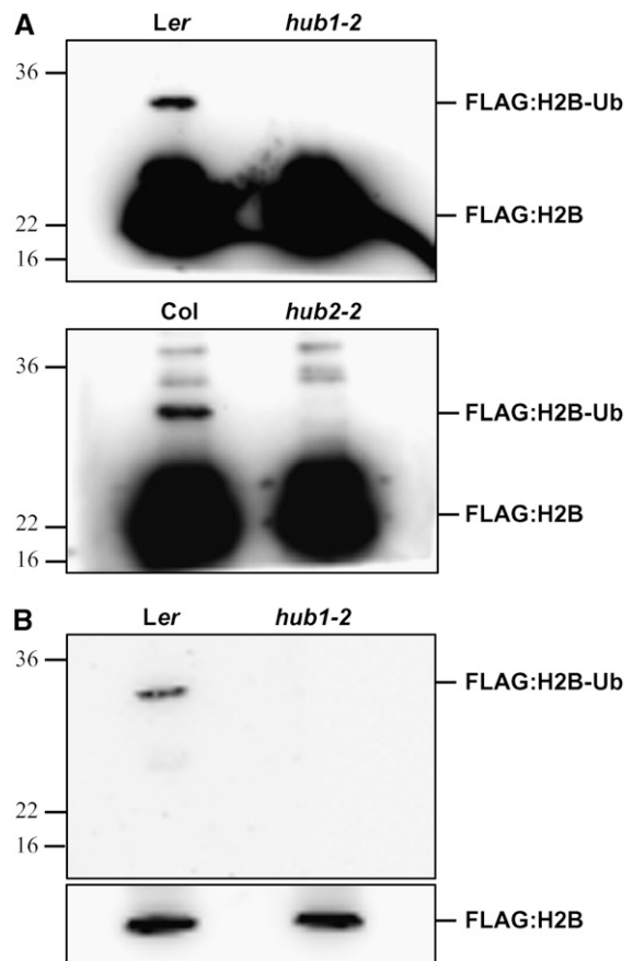
Figure 7. In Vivo Analysis of Histone H2B Monoubiquitination.
