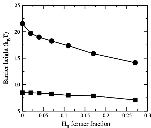
FIGURE 5 Barrier height of fusion process as a function of the volume fraction of the hexagonal-forming ( H_{II} ) amphiphile. The upper curve shows the barrier heights in the standard stalk-hemifusion mechanism. The lower curve shows the barrier heights in the first stalk-hole mechanism with a defect energy of F_d = 4 k_B T .
