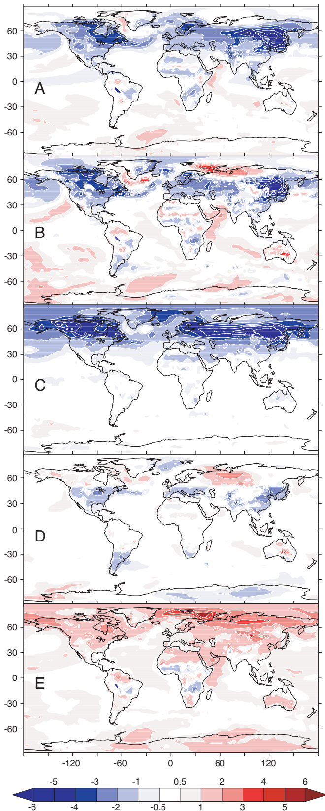
Fig. 3. Simulated spatial surface temperature differences relative to the Standard experiment in the decade centered on year 2100 for the Global ( A ) and linear sum ( B ) of Boreal ( C ), Temperate ( D ), and Tropical ( E ) deforestation experiments. Cooling biophysical effects of deforestation overwhelm warming carbon-cycle effects over most of the land surface (including tropical regions), but are most pronounced in the Northern high latitudes. Comparison
