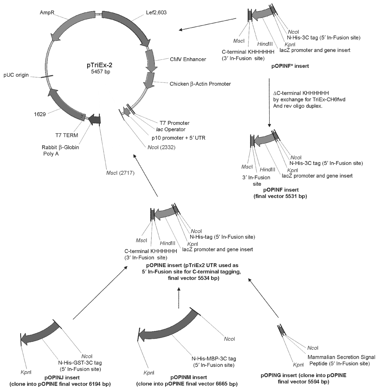
Figure 1. Vector derivations and maps. Derivation of the pOPIN vectors from pTriEx2. PCR fragments were prepared as described in the Materials and methods section and either ligated into the pTriEx2 vector or inserted by In-Fusion TM . In cases where the pOPIN vector is not directly derivatized from pTriEx2, the intermediate vector is also shown. Features of the pTriEx2 vector retained in the pOPIN vector suite are: T7/ lac O promoter/operator and terminator for inducible expression in E. coli harbouring the \lambda (DE3) prophage, CMV Enhancer/Chicken \beta -actin promoter and rabbit \beta -globin polyA site for efficient expression in mammalian hosts, p10 baculoviral promoter and 5' UTR/ORF603 and ORF 1629 for efficient expression from/recombination into baculovirus respectively. The high-copy pUC origin of replication and \beta -lactamase (Ampicillin resistance marker) gene allow high-copy production of the vector in E. coli .
