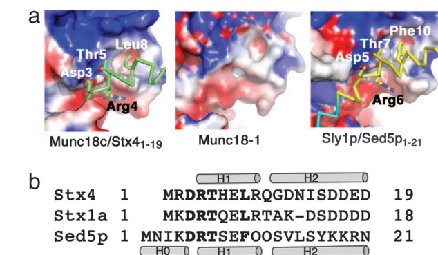
Fig. 3. A structurally conserved N-peptide binding site in Munc18c, Sly1p, and Munc18-1. (a) Electrostatic surfaces are shown for the structures of Munc18c, Munc18-1, and Sly1p in the N-peptide binding region (colored blue to red from +5 to -5 KbT/e). An acidic groove (red), basic patch (blue), and hydrophobic pocket (white) characterize the N-peptide binding sites of Munc18c and Sly1p, and these features are also present in Munc18-1. The main chain of the N-peptides of Stx4 (green) and Sed5p (yellow and blue) and the side chains of the DRT motif and hydrophobic residues are shown. (b) Sequence alignment of the N-peptides of mouse Stx4, rat Stx1a, and yeast Sed5p is shown with the DRT motif and hydrophobic residue indicated in bold. Helices are shown as cylinders for Stx4 and Sed5p.
