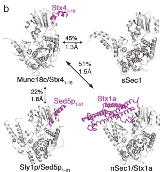
Fig. 1. Structure of Munc18c/Stx4 1–19 and comparison with other SM proteins. (a) The Munc18c/Stx4 1–19 complex showing domain 1 (residues 1–138) in dark blue, domain 2 (residues 139–250 and 476–584) in orange, and domain 3 (residues 251–475) in cyan. Stx4 residues 1–19 are shown in magenta. Helices are shown as coils, and strands are shown as arrows. N and C termini and secondary structure elements are labeled. (b) Comparison of mouse Munc18c/Stx4 1–19 with squid neuronal Munc18-1 [sSec1, PDB ID code 1EPU (23)], yeast Sly1p/Sed5p 1–21 [PDB ID code 1MQS (20)], and rat neuronal Munc18-1/Stx1a [nSec1/Stx1a] [PDB ID code 1DN1 (10)] showing rmsd of the structures and the pairwise sequence identity.
