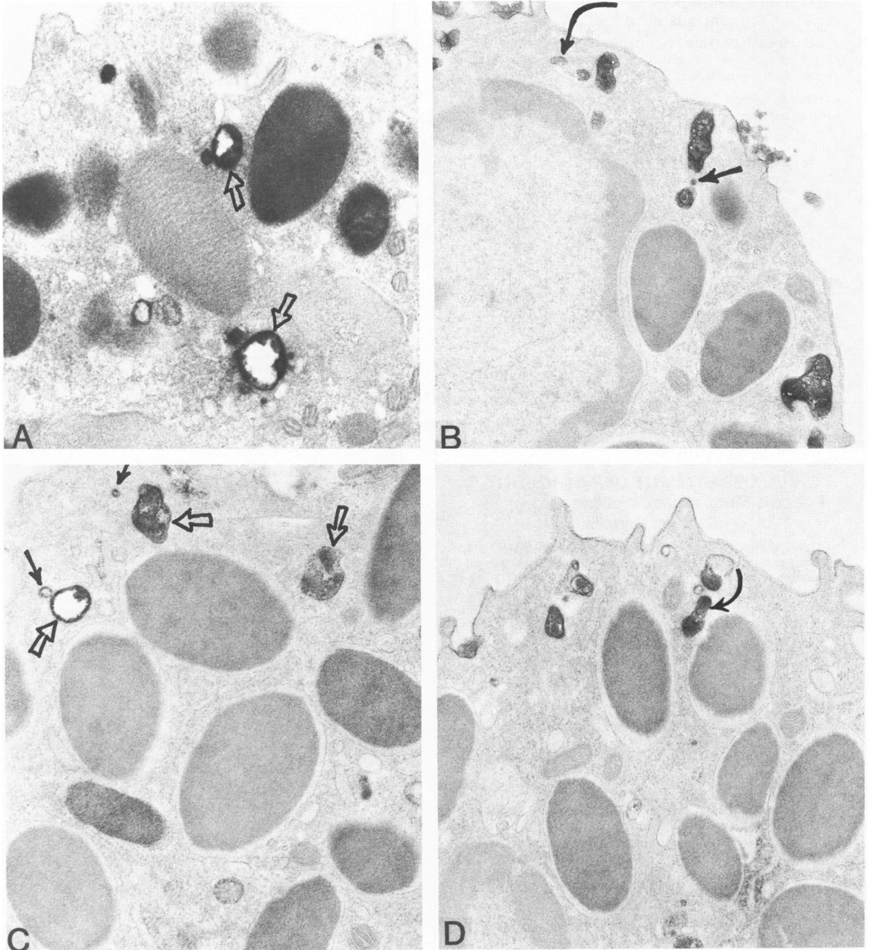
Figure 2 —Guinea pig basophils reacted for peroxidase content after exposure to EPO for 15 minutes (A) or 30 minutes (B–D). Note positive cytoplasmic vesicles (solid arrows), vacuoles (open arrows), and tubules (curved arrows). In these cells, most of the granules are peroxidase-negative, but several are strongly positive (A). (A, \times 25,000 ; B, \times 22,000 ; C, \times 27,500 ; D, \times 25,000 )
