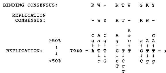
FIG. 7. Summary of replication data and a derived consensus sequence for the 18-bp IR half site. Shown in bold capitals is the wild-type BPV-1 sequence from nucleotides 7940 to 3, which constitutes the 5' half of the 18-bp IR element. Individual nucleotide changes that replicated at ≥50% of wild-type levels are shown above the wild-type sequence, while mutations that reduced replication to <50% of wild-type levels are shown below. Mutations from both half sites were combined into a single half site for evaluative purposes as discussed in the text. Mutations derived from the 5' and 3' halves of the 18-bp IR are given in uppercase and italicized lowercase letters, respectively. Above the mutations is the consensus sequence for nucleotides critical for replication function. This consensus was derived from the available mutations that replicated at ≥50% of wild-type levels. The dash in the consensus sequence indicates that at least three different nucleotides could occupy that position and maintain near wild-type replication. Above the replication consensus sequence is the binding consensus sequence derived in a similar fashion from the binding data in Fig. 4A.
