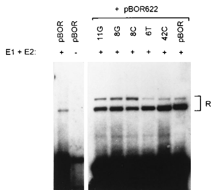
FIG. 6. Representative transient DNA replication of pBOR and origin mutations. Transient replication assays were performed as described in Materials and Methods with C127 cells, and a representative Southern blot is shown. The E1 and E2 expression vectors were included (+) or excluded (-) as indicated. Plasmid pBOR622 was coelectroporated with certain samples as indicated by the bracket above lanes 3 to 8. DNA was harvested at either 3 days (lanes 1 and 2) or 5 days (lanes 3 to 8) postelectroporation and was digested with DpnI and HindIII . The position of the linear, DpnI -insensitive (replicated) DNA is indicated by the bracket and R to the right. In each lane, the upper replicated band corresponds to pBOR622 and the lower band corresponds to the pBOR clone. Designations above lanes 3 to 7 indicate the BPV-1 nucleotide position and the nucleotide change of the mutations being tested. Note that 42C corresponds to BPV-1 nucleotide 7942.
