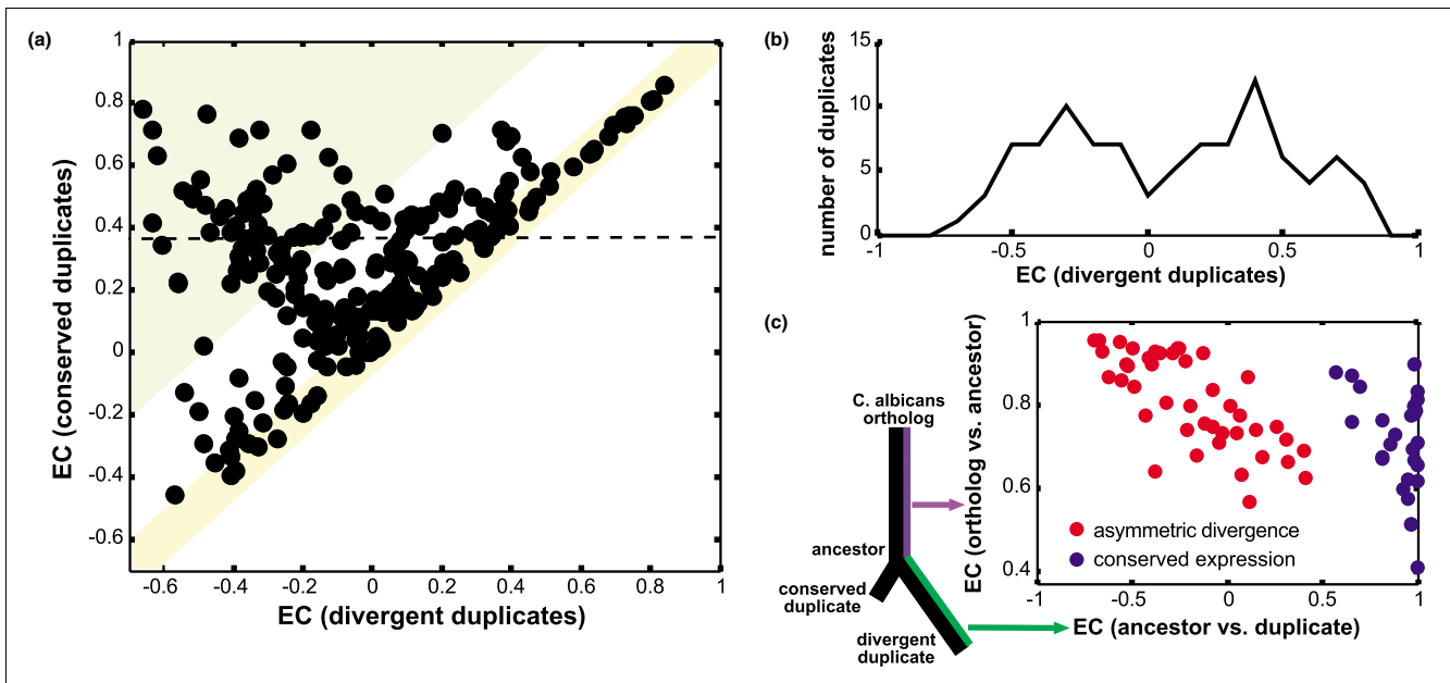
Figure 3 Expression conservation between duplicates and their ancestors. (a) Each dot represents the EC of a duplicate pair where the EC of the less conserved duplicate is shown on the x-axis and the EC of the more conserved duplicate is shown on the y-axis. The yellow region indicates similar rates of expression divergence ( y - x < 0.2 ) and the green region indicates asymmetric rates of expression divergence ( y - x > 0.5 ). The dashed line indicates a threshold of EC > 0.37 , which is the 0.05 significance value from randomly selected S. cerevisiae - C. albicans gene pairs (see Figure 2b). (b) Distribution of EC for the least conserved duplicates among the 96 cases where the more conserved duplicate has significantly high EC (above the dashed line in (b)). (c) EC between the least conserved duplicate and the reconstructed ancestral expression (x-axis), and between the C. albicans ortholog and the reconstructed ancestral expression (y-axis). Red dots correspond to duplicates with asymmetric expression divergence (left peak in (b)) and blue dots correspond to duplicates with conserved expression (both copies with EC > 0.37 ).
