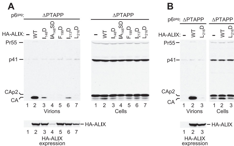
FIG. 3. Effects of mutations targeting surface patch 1 of the ALIX Bro1 domain on the ability of ALIX to rescue virion release by \Delta PTAPP HIV-1. (A) 293T cells were transfected with the \Delta PTAPP mutant (1 \mu g) and vectors expressing WT HA-ALIX or the indicated mutants, or empty vector (2 \mu g). Virion production and the expression levels of Gag and HA-ALIX were monitored by Western blotting. (B) Comparison of the abilities of WT and L 216 D ALIX to rescue virion release when expressed at similar levels. 293T cells were transfected with the \Delta PTAPP mutant (1 \mu g) and vectors expressing WT HA-ALIX (2 \mu g), L 216 D HA-ALIX (4 \mu g), or empty vector (2 \mu g).
