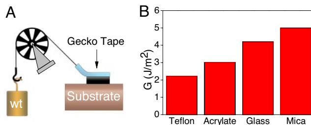
Fig. 4. Peeling measurements of the gecko tapes on various substrates. We performed the peeling measurements at different angles using the setup shown in A. (B) The energy of detachment, G ( \text{J}/\text{m}^2 ), plotted at a peeling angle of 45° on various substrates.
