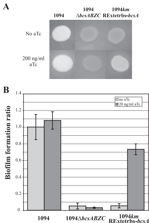
FIG. 6. Modulation by the REXtETTrbs cassette of cellulose production and biofilm formation by an E. coli natural isolate. The ability of the different 1094-derivative strains to produce cellulose was tested. (A) Calcofluor binding and fluorescence under UV light. Two-microliter volumes of overnight cultures were spotted onto LB-calcofluor (upper row) and LB-calcofluor-aTc (lower row) plates and incubated for 24 h at 37°C; the aTc concentration on the plate was 200 ng/ml. (B) Capacities for the formation of biofilms in microfermentors. Biofilms were grown for 26 h at 37°C in M63B1glu supplemented or not with 20 ng of aTc/ml. The levels of biofilm formation by the different strains are expressed as the ratios of the OD readings for the resuspended biofilms of the different strains to that for the 1094 biofilm in the absence of aTc. Data are averages of results from three independent experiments; error bars represent standard deviations of the means.
