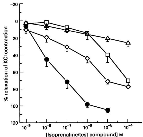
Figure 4 Concentration-response curves to (–)-isoprenaline and pindolol analogues in rat ileum precontracted with 40 mM KCl. Relaxation was induced by (–)-isoprenaline (●), and with descending potencies by iodocyanopindolol (◇) and cyanopindolol (□). Pindolol (△) did not cause relaxation significantly different from that produced by the solvent (DMSO). CGP 20712A and ICI 118 551 ( 0.1 \mu\text{M} ), atropine ( 0.5 \mu\text{M} ) and corticosterone ( 100 \mu\text{M} ) were present in all preparations. n = 4 to 5.
