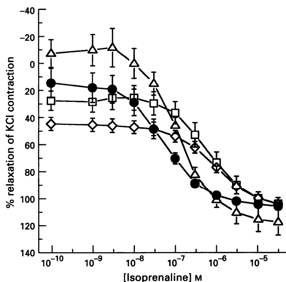
Figure 5 Concentration-response curves to (-)-isoprenaline (●) in rat ileum precontracted with 40 mM KCl, in the presence of pindolol (△), cyanopindolol (□) and iodocyanopindolol (◇). CGP 20712A and ICI 118 551 (0.1 μM), atropine (0.5 μM) and corticosterone (100 μM) were present in all preparations. n = 4 to 5.
