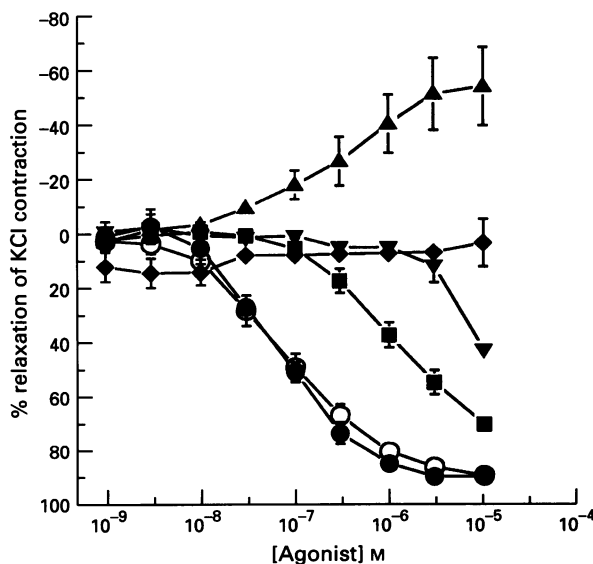
Figure 2 Concentration-response curves for various compounds in rat ileum precontracted with 40 mM KCl. (–)-Isoprenaline produced almost identical relaxation in ileum obtained 20 cm proximal to the caecum (○) and immediately proximal to the caecum (●). Relaxation was also induced by the \beta_1 -selective agonist, RO363 (■), and the \beta_2 -selective agonist salbutamol (▽). The \alpha -agonist (–)-phenylephrine (◆) did not cause relaxation, and 5-HT (▲) caused contraction. CGP 20712A and ICI 118 551 ( 0.1 \mu\text{M} ), atropine ( 0.5 \mu\text{M} ) and corticosterone ( 100 \mu\text{M} ) were present in all preparations. n = 4 .
