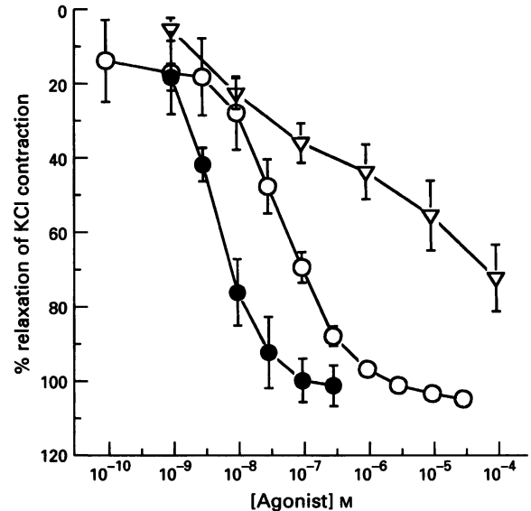
Figure 3 Concentration-response curves to various \beta_3 -agonists in rat ileum precontracted with 40 mM KCl. (–)-Isoprenaline (○) and BRL 37344 (●) were both potent full agonists, whereas ICI D7114 (▽) was only a partial agonist with a lower potency. CGP 20712A and ICI 118 551 ( 0.1 \mu\text{M} ), atropine ( 0.5 \mu\text{M} ) and corticosterone ( 100 \mu\text{M} ) were present in all preparations. n = 4 .
