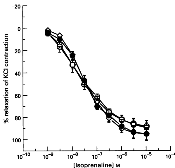
Figure 1 Concentration-response curves to (-)-isoprenaline in rat ileum precontracted with 40 mM KCl. Experiments were conducted in the absence of CGP 20712A and ICI 118 551 (○), in the presence of 0.1 μM CGP 20712A (□), 0.1 μM ICI 118 551 (◇), or 0.1 μM CGP 20712A and ICI 118 551 (●). Atropine (0.5 μM) and corticosterone (100 μM) were present in all preparations. n = 4 to 5.
