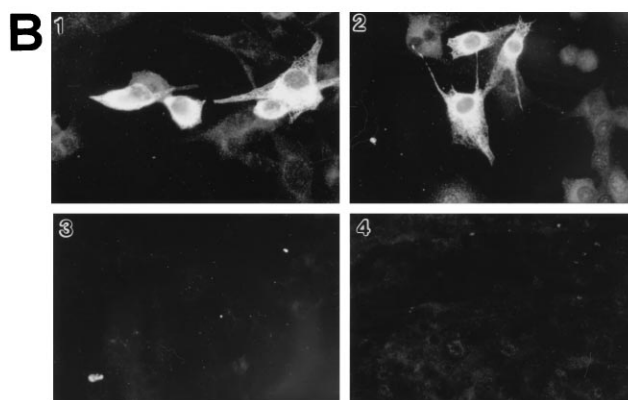
FIG. 3. In vitro translation and immunofluorescence analyses of replicon RNAs with deletions in the C coding sequence. (A) In vitro translation of deleted RNAs in rabbit reticulocyte lysates. RNA transcripts were prepared from the corresponding cDNAs digested with Eco RI at nucleotide 3924 of KUN cDNA (in codon 133 of the NS2A protein) and translated in rabbit reticulocyte lysates (Promega) supplemented with [ ^{35}\text{S} ]methionine/cysteine for 60 min at 30°C. Radiolabelled translation products were identified by autoradiography after electrophoretic separation in a 10% polyacrylamide gel; positions of prestained molecular weight markers (Bio-Rad) are shown on the left. (B) Immunofluorescence with anti-NS3 antibody of BHK21 cells at 24 h after electroporation with \Delta ME/76(C107rep) and C20rep RNAs (panels 1 and 2, respectively) and at 48 h after electroporation with C2rep RNA (panel 3) or mock-electroporated BHK cells (panel 4). Transfected cells on coverslips were fixed with acetone at -20^\circ\text{C} for 30 s, air dried, and incubated with rabbit anti-NS3 antibody at room temperature for 30 to 60 min and subsequently with fluorescein isothiocyanate (FITC)-conjugated goat anti-rabbit immunoglobulin G (IgG) for 30 min.
