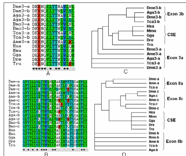
Figure 1 Multiple alignments and phylogenetic analysis of duplicated exon nucleotide sequences. (A, B) Multiple alignments of amino acid sequences of duplicated exon 3 (A) and exon 8 (B) sequences and their counterparts from orthologs in other species, respectively. The alternative exons are labeled 'a' and 'b' or 'c'. (C, D) Cladogram of insect duplicated exon DNA sequences and vertebrate orthologous constitutive exons corresponding to the alignments shown in (A, B). For each cluster, the amino acid sequences of each alternative exon from each species were aligned using the Clustal W program and phylogenetic trees generated. The branches contained the vertebrate constitutive exons (CSE), invertebrate alternative exons 8a or exons 3a, alternative exons 8b or exons 3b and alternative exons 8c, respectively. Abbreviations: Hsa, H. sapiens (NM_000746.3); Dre, D. rerio (NP_957513.1); Mmu, M. musculus (NP_031416.2); Gga, G. gallus (NP_989512.1); Tru, T. rubripes (CAG03274.1); Dme, D. melanogaster (CG4128) [16]; Aga, A. gambiae [17]; Bmo, B. mori (CH379590); Tca, T. castaneum (CM000280); Ame, A. mellifera [21].
