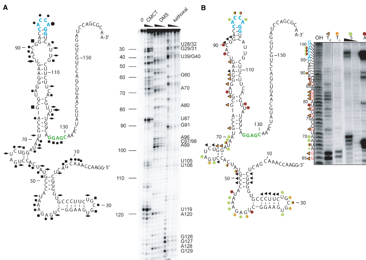
Figure 2. Proposed secondary structure of the TPP-free form of the thiM riboswitch from E. coli . The sequence complementary to and binding to the previously selected hairpin N25.1.22 is shown in cyan. The SD-sequence is highlighted in green. (A) Secondary structure of the TPP-free form of the thiM riboswitch (left panel) as well as primer extension reactions after chemical modifications of the riboswitch with CMCT, DMS or kethoxal (right panel). Positions that are chemically modified are marked with symbols (DMS, black dot; kethoxal, black square; CMCT, black diamond). Untreated RNA is referred to as 0. (B) Secondary structure of the TPP-free form of the thiM riboswitch (left panel) as well as enzymatic probing data (right panel) including the cleavage pattern of 5'-[ 32 P]-labeled 165 thiM by alkaline hydrolysis (OH) and different nuclease digestions (denaturing T1, T d , native T1, T n , S and A). Labels are: RNase S, green hexagons; RNase A, red hexagons; RNase T1 native, orange hexagons; RNase T1 denatured, black bordered orange triangles.
