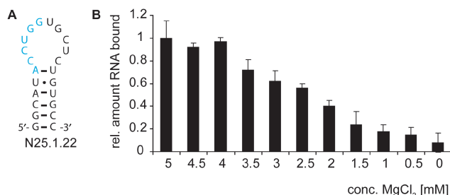
Figure 1. The in vitro selected hairpin N25.1.22 binds to the TPP-free form of the 165 thiM riboswitch in a Mg 2+ -dependent manner. (A) Primary sequence of the selected hairpin N25.1.22. The sequence which is complementary to the thiM riboswitch is highlighted in cyan. (B) Binding of the hairpin N25.1.22 to the thiM riboswitch is dependent on the concentration of Mg 2+ -ions in the reaction.
