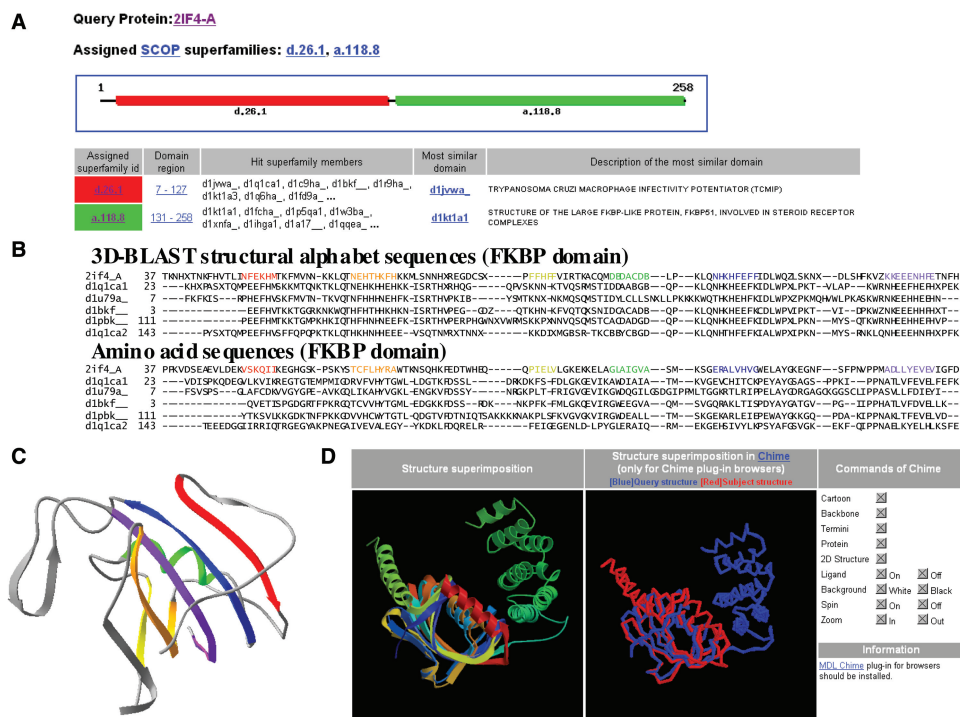
Figure 2. Evolutionary superfamily assignment and structural alignment of the fastSCOP server using the structure of multi-domain immunophilin ( AtFKBP42 ) from Arabidopsis thaliana (PDB code 2IF4-A) as the query. (A) The assigned SCOP superfamilies are the FKBP-like domain (SCOP entry d.26.1) and the TPR domain (SCOP entry a.118.8). (B) Multiple structural alphabet and amino acid sequences alignments of FKBP-like domain between the query protein and five homologous proteins. The aligned secondary structures are represented as a continuous color spectrum from red through orange, yellow, green and blue to violet. The color is mapped to (C) the structure of the FKBP-like domain. (D) Structural alignments between the FKBP-like domain of the query protein and that of the homologous protein (PDB code 1Q1C-A).
