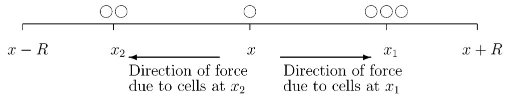
Fig 2. A schematic illustration of cell movement under an attractive force towards cells at position x .
