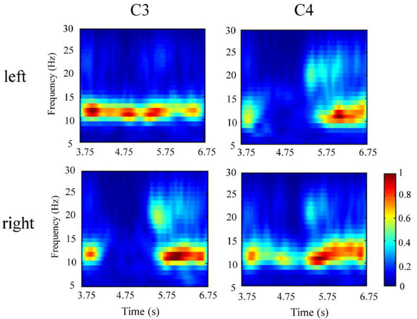
Fig. 2. Averaged Time-Frequency (TF) representation of channel C3 and C4 during motor imagery in a subject. Left column refers to TF representation for C3 and right column for C4. The upper row refers to the TF representation of left hand movement imagination and the lower refers to right hand movement imagination. The time period shown here is 3s from the preparation cue (3.75s) and frequency band is from 5 to 30 Hz.
