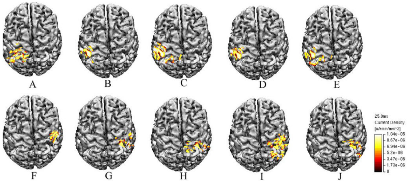
Fig. 5. Examples of cortical current density distributions of different trials in a human subject during motor imagination. (A,B,C,D,E - left-hand movement imagery; F,G,H,I,J – right-hand movement imagery). Results were estimated from single trial scalp EEG data. See text for detailed procedures to obtain single trial inverse solutions.
