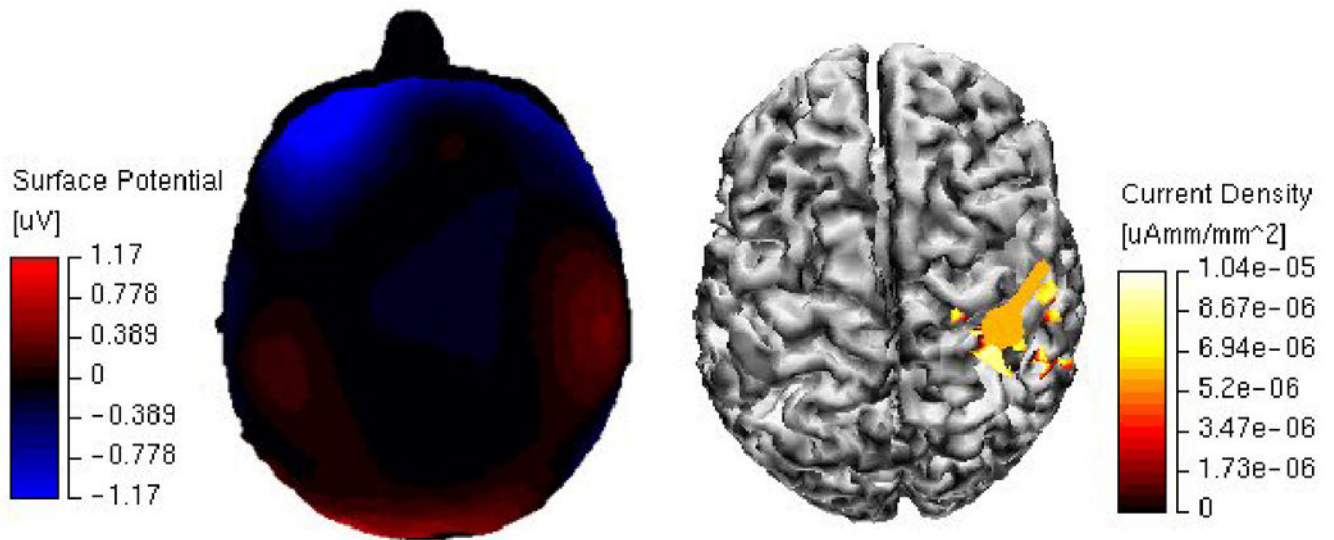
Fig. 3. Illustration of effect of source analysis. The left panel illustrates the surface Laplacian and temporal-bandpass filtered scalp EEG map of a single trial, and the right panel depicts the equivalent dipole solution and cortical current density distribution estimated from it.
