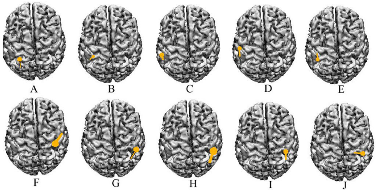
Fig. 4. Examples of equivalent dipole solutions of different trials in a human subject during imagination of left or right hand in alpha band. (A,B,C,D,E - left-hand movement imagery; F,G,H,I,J - right-hand movement imagery). Results were estimated from single trial scalp EEG data. See text for detailed procedures to obtain single trial inverse solutions.
