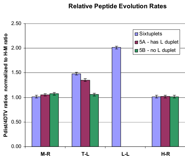
Figure 3 Normalized peptide to nucleotide evolutionary rates show an accelerated divergence of duplicated X. laevis peptides. The chart shows the ratio of peptide evolution (P-distance) to synonymous transversion rates (4 DTv), normalized by the human-mouse P-distance/4 DTv value of 0.242 \pm 0.004 , for three sets of multiple alignments corresponding to genes found in single copy in each of human, mouse, rat, and X. tropicalis , and two copies in X. laevis (sextuplets); pentuplets obtained by randomly selecting one X. laevis paralog from each sextuplet (5 A), and pentuplets in which only a single X. laevis sequence is known (5B).
