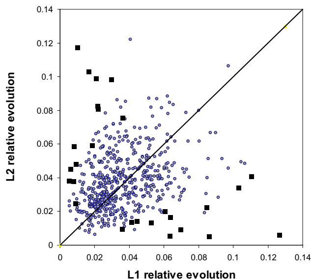
Figure 2 Symmetric evolution of paralogs. Scatter plot of relative evolution between X. tropicalis peptides and their co-orthologous sequences in X. laevis . A total of 578 gene triples with 16 or more highly-conserved positions are shown (see text for details). L1 and L2 refer to co-orthologous genes 1 and 2 in X. laevis . The diagonal line represents a null model assuming symmetric evolution of L1 and L2. Black boxes are L1–L2 pairs inconsistent with this model at P < 0.01 .
