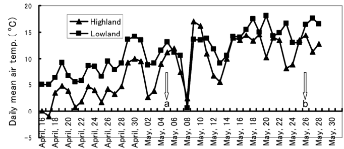
Figure 1. The daily mean air temperature (°C) during sampling of the experimental areas. a, b; date of sampling at lowlands and highlands, respectively.
