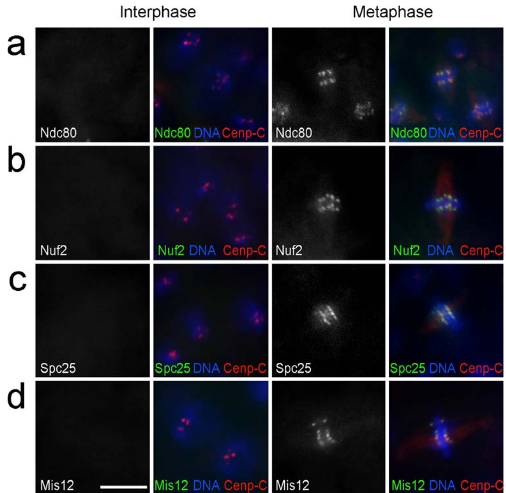
Fig. 1 Localization of Drosophila Ndc80 complex components and Mis12. Transgenic embryos expressing EGFP fused to either a Ndc80, b Nuf2, c Spc25, or d Mis12 were fixed at the stage when some cells progress through the 14th, asynchronous round of mitosis. Cells in interphase ( left panels ) and metaphase ( right panels ) after double labeling with an antibody against Cenp-C (Cenp-C) and a DNA stain (DNA) illustrate that the EGFP fusion proteins were only associated with centromeres during mitosis. Bar=5 \mu m
