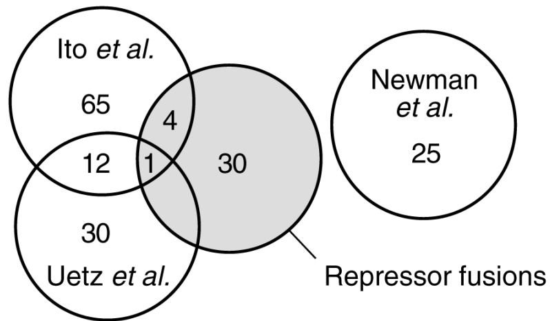
Figure 4. Venn diagram showing homotypic interactions found in three large-scale two-hybrid projects and our repressor fusion libraries. The homotypic interaction subset from Ito et al. (2001) was extracted from the full dataset ( http://genome.c.kanazawa-u.ac.jp/Y2H/ ). The homotypic interaction subset from Uetz et al. (2000) was extracted from ( http://depts.washington.edu/sfields/yplm/data/ )
