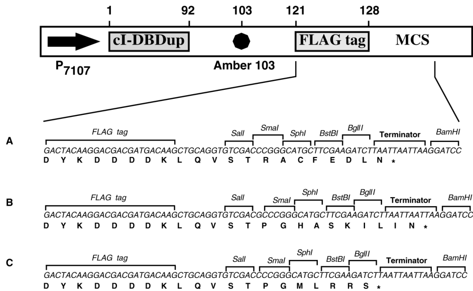
Figure 5. Schematic representation of repressor fusion vectors used in this study. A. Sequence of the multiple cloning site region in pLM99. B. Sequence of the multiple cloning site region in pLM100. C. Sequence of the multiple cloning site region in pLM101
