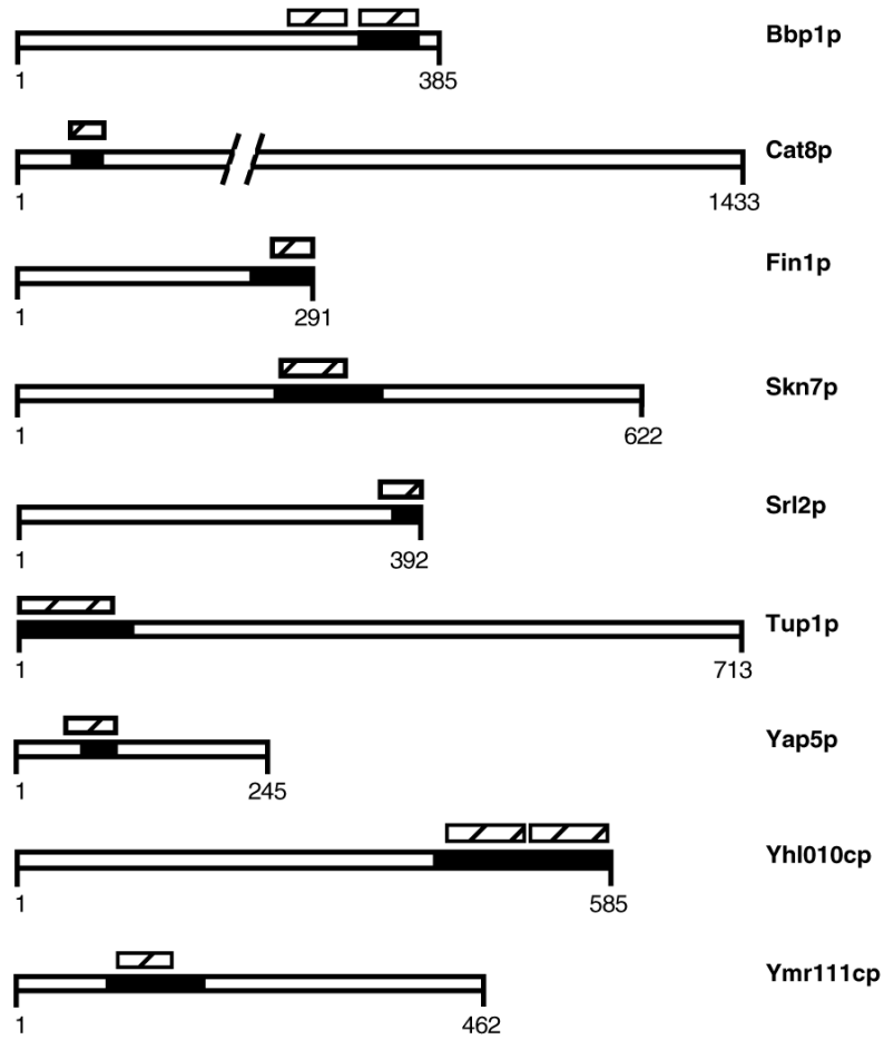
Figure 3. Predicted coiled-coils in proteins containing ISTs. The location of the minimal IST is represented by the black boxes. The slashed boxes represent regions predicted to contain a coiled coil region by COILS ( http://tofu.tamu.edu/COILS2/ ). The predicted regions have coiled-coil probabilities >0.8 in COILS
