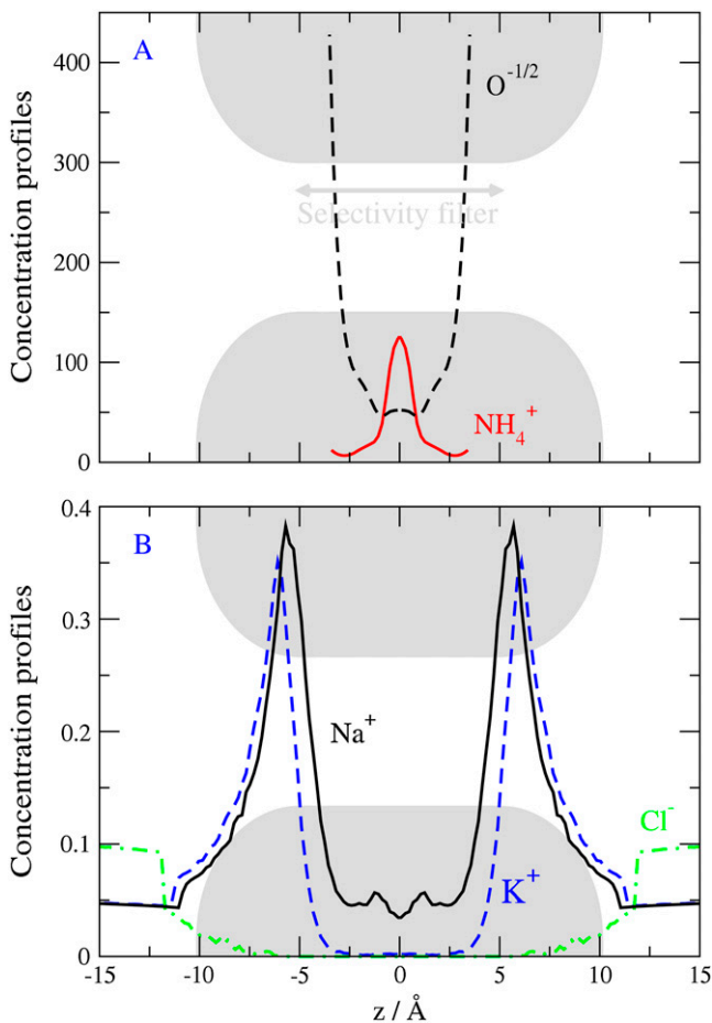
FIGURE 6 Longitudinal concentration profiles for various ions in the DEKA Na channel (charge = -1e ). R = 3\text{Å} , \epsilon_p = 10 , and [\text{NaCl}] = [\text{KCl}] = 0.05\text{ M} . This figure shows selectivity by depletion within the filter and binding outside the filter. The binding is not selective and occurs because the pressure arising from the excluded volume of ions and side chains forces the counterions to dwell near rather than in the filter region. Counterions accumulate at the filter entrances to the filter because they are electrostatically attracted to it but they cannot fit within the filter. This is an essential feature of the charge-space competition mechanism of selectivity.
