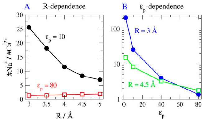
FIGURE 10 The ratio of the occupancies of Na + and Ca 2+ ions (A) as a function of pore radius R for two different protein dielectric coefficients of the protein ( \epsilon_p = 10 and 80) and (B) as a function of \epsilon_p for two different radii of the pore ( R = 3 and 4.5 Å). The bath Ca 2+ concentration is 17.5 mM. Protein dielectric coefficient has little effect on Na + versus Ca 2+ selectivity when the protein dielectric coefficient is large, but it has a substantial effect when the protein dielectric coefficient is small. The radius of Na + and Ca 2+ are nearly the same ( \text{Na}^+ = 1 , \text{Ca}^{2+} = 0.99 Å) so this graph shows charge selectivity. The selectivity filter has spatially nonuniform selectivity (see Fig. 7) and so we define and plot occupancy in the central most-selective region of the filter \pm 2.5 Å from the center of the pore.
