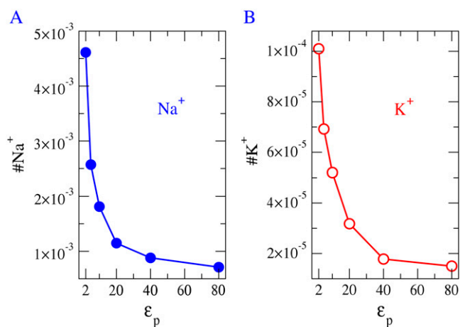
FIGURE 9 The occupancies of Na + and K + ions as a function of \epsilon_p for R = 3 Å. The electrolyte is equimolar: [\text{NaCl}] = [\text{KCl}] = 0.05 M. The protein dielectric coefficient has a large effect on occupancy and thus (most likely) on the conductance of the channel even though it has little effect on the selectivity, i.e., the ratios of occupancies seen in Fig. 7 A, left-hand panel. The selectivity filter has spatially nonuniform selectivity (see Fig. 7) and so we define and plot occupancy in the central most selective region of the filter \pm 2.5 Å from the center of the pore.
