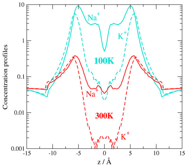
FIGURE 11 Longitudinal concentration profiles for Na + and K + ions in the DEKA locus for crystallographic temperature 100 K (blue lines) and biological temperature 300 K (red lines). Pore radius is R = 3 \text{ \AA} , protein dielectric coefficient is \epsilon_p = 10 , and [\text{NaCl}] = [\text{KCl}] = 0.05 \text{ M} , the same situation as in Fig. 5. Note the profound effect of temperature. Barriers and wells are frozen into the structure at crystallographic temperatures because entropy is low. The profile shows little such structure at biological temperature where entropic disorder is much larger. Measurements made at one temperature give qualitatively different results from those at another.
