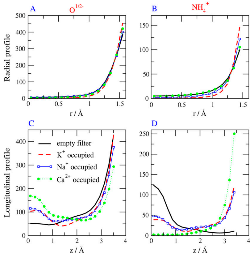
FIGURE 4 The effect of ion contents in profiles in a DEKA Na channel. (A,C) Distribution of O^{1/2-} ; (B,D) Distribution of NH_4^+ . The selectivity filter has spatially nonuniform selectivity (see Fig. 7) and so we define and plot occupancy in the central most selective region of the filter \pm 2.5 \text{\AA} from the center of the pore. This region is either occupied by one Na^+ ion; or one K^+ ion; or one Ca^{2+} ion; or the filter is empty. The longitudinal distribution of side chain structural ions ( O^{1/2-} and NH_4^+ ) is shown in the lower two panels of C and D. The radial distribution of side chains is shown in the upper two panels of A and B. Filters labeled empty contained side-chain structural ions but no Na^+ , K^+ , or Ca^{2+} ion.
