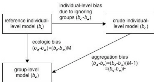
Figure 9 Bias magnification and inflation. The ecologic bias ( b_e - b_w ) equals the individual-level bias ( b_c - b_w ) – due to confounding by group and effect modification of the risk difference by group – multiplied by the magnification factor M , assuming no other sources of ecologic bias. The ecologic bias also equals the sum of the individual-level bias due to ignoring groups and the bias caused by aggregation. The latter is measured by F , the inflation factor, equal to M - 1 .
