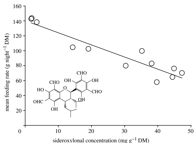
Figure 2. Effect of sideroxylylonal concentrations on feeding rates of koalas fed E. melliodora foliage, from a linear mixed model (Wald statistic = 20.63, d.f. = 1, p < 0.001 ). Open circles indicate mean koala intakes for 12 trees, adjusted for random effects (koala, tree, koala \times night). Inset: sideroxylylonal A.
