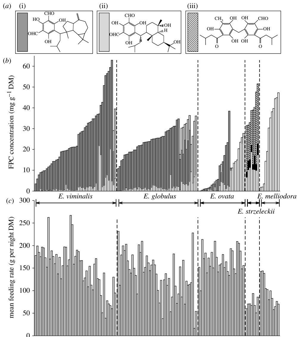
Figure 1. (a)(i) Macrocarpal G; (ii) macrocarpal I; and (iii) jensenal. (b) Stacked bar charts indicating the concentrations of sideroxytonals (open bars), ‘Group 1’ macrocarpals (dark grey), ‘Group 2’ macrocarpals (light grey), grandinal (black) and jensenal (diagonally hatched) in 150 trees of five species fed to koalas. (c) Bar chart indicating mean amounts of foliage eaten by koalas from the trees indicated above.
