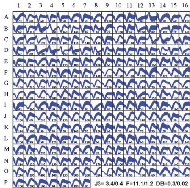
Fig. 4. Samples of action potentials from 247 single neurons recorded in monkey 3, 30 days after implantation. Sample includes left M1 (A1–F7), left PMd (F8–H7 and J3–K7), left S1 (H8–J2), right S1 (K8–N11), and right M1 (N12–P7). Numbers next to the sampled waveforms display their Vpp ( \mu\text{V} ). Mean \pm SE J3 (2D), F (2D), and DB (2D) statistics for the sample are plotted at the bottom right.
