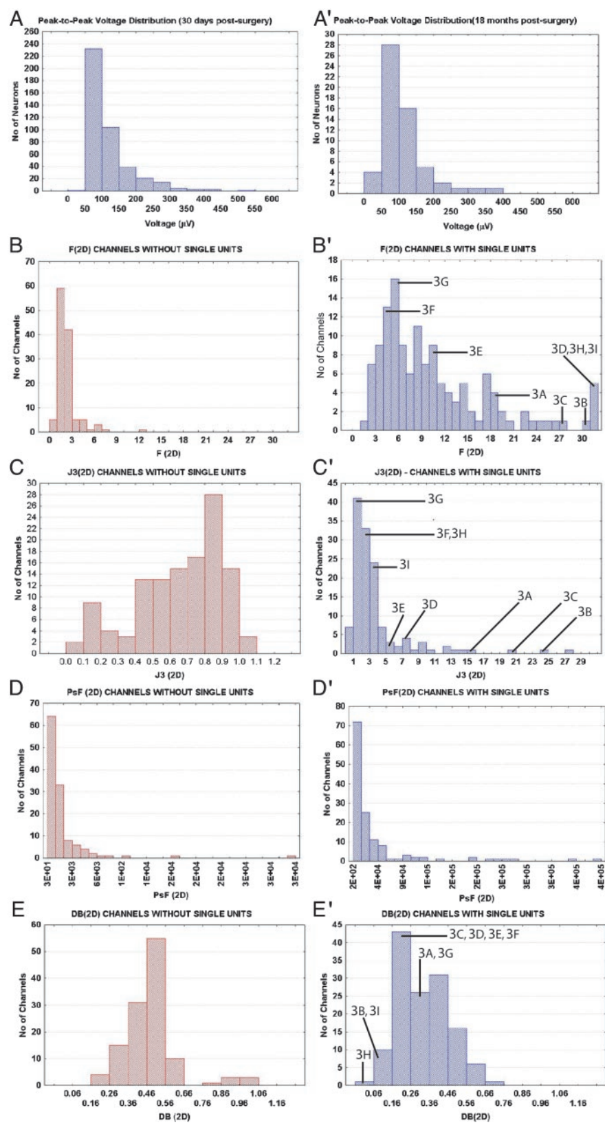
Fig. 3. (A) Vpp distribution from 330 single neurons recorded in two monkeys, 30 days after the surgical implantation. (A') Vpp distribution obtained for monkey 1, 18 months postsurgical implantation. Distributions of four cluster separation statistics for channels without isolated single units (B–E) and with single units (B'–E'). (B) Distribution of F (2D) values for recording channels without single units. (B') Distribution of F (2D) values for channels with single units. The locations in the distribution of the channels are indicated by labels and lines. (C) Distribution of J3 (2D) values for channels without single units. (C') Distribution of J3 (2D) values for channels with single units. (D) Distribution of PsF (2D) values for channels without single units. (D') Distribution of PsF (2D) values for channels with single units. (E) Distribution of DB (2D) values for channels without single units. (E') Distribution of DB (2D) values for channels with single units.
