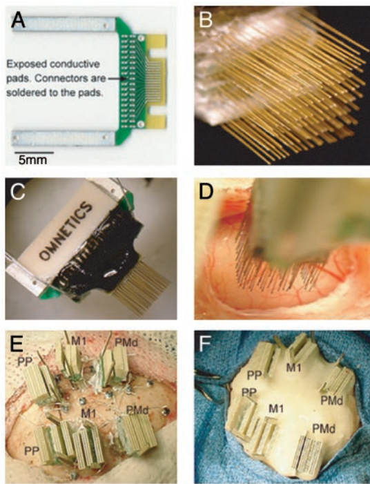
Fig. 1. (A) Printed circuit board (PCB) used to build a high-density microwire array (spacing between traces is 300 \mu\text{m} ). (B) Multiple boards are stacked up to form arrays with up to 128 microwires. (C) High-density connectors are attached to the other side of the board. (D) Implantation of a 128-microwire array in the M1. (E) Last stages of a 672-microwire implant. Bilateral implants included the PMd, M1, and the PP. (F) Final aspect of a multisite implant after the application of multiple layers of dental cement.
