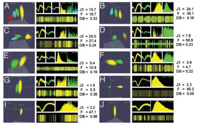
Fig. 2. Examples of cluster separation, 30 days postimplantation. Each example contains: (Left) identified clusters in 3D PC space; (Upper Middle) waveforms; (Upper Right) ISI histograms; (Lower Right) continuous record of potentials. Different colors depict distinct clusters in all parts of each example. J3 (2D), F (2D), and DB (2D) statistics are at the far right. (A) Three single units (yellow, green, and blue) discriminated from the multiunit record (red cluster) yielded high J3 and F values, average DB, clear differences in waveforms, and ISI histograms. (B) Two single units (green and yellow) were differentiated from the multiunit activity (blue), producing high J3 and F and low DB values. (C) High separation between the multiunit cluster (blue) and two units (yellow and green). (D) One large (yellow) and one small (green) unit were isolated from the multiunit activity (blue). (E) Two clearly distinct units were isolated. J3 was above the mean, DB was good, and F value was average. (F) Two units with distinct amplitudes and ISI histograms from a channel with below average J3 and F values. The DB value indicates good cluster separation. (G) Channel with low J3 and F values, but an average DB. Two units with distinct waveforms and ISI histograms were isolated. (H) Example of a large single unit (yellow) isolated from the multiunit activity (green). J3 was below average, F was very high, and DB was very low. (I) Single unit (yellow) clearly distinct from the multiunit activity (green). The J3 value was close to its mean, the F value was high, and DB was low, indicating excellent cluster separation. (J) A single unit (yellow cluster) isolated way above the multiunit voltage level. ISI histogram time scales were 5 ms (C), 10 ms (A, D, and G), and 100 ms (B, E, F, and H–J).
