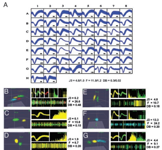
Fig. 5. (A) Waveform sample from 58 single neurons recorded 18 months after the implantation surgery. Numbers next to waveforms depict the mean Vpp ( \mu\text{V} ) of the action potentials. Right PMd (A1–B2), right M1 (B3–E6), right S1 (E7–F7), and right SMA (F8–H2). Mean \pm SE J3 (2D), F (2D), and DB (2D) statistics for the sample are plotted at the bottom right. (B–G) Single neuron isolation quality is illustrated as described in Fig. 3. (B) Four single units discriminated from the multiunit activity (blue). (C) Clear isolation of a single neuron (yellow) from the multiunit activity (green) is confirmed by high J3 and F values and a low DB. (D) Channel with a clear single unit, but with a smaller signal-to-noise ratio than C. ISI histograms show a clear refractory period. (E) Two clearly distinct single units produced clusters with average J3, close to average F, and low DB. (F) Two units (green and yellow) discriminated from the multiunit activity (blue) yielding high J3, F, and low DB statistics. Distinct ISIs, waveform shapes, and amplitudes further supported their designation as single units. (G) Channel with average J3 and slightly lower than average F and DB statistics. Clear differences in ISI histograms and waveform shape and amplitude confirm nice separation of units (green and yellow) from multiunit activity (blue). ISI histogram time scales are 10 ms (B–F) and 100 ms (G).
