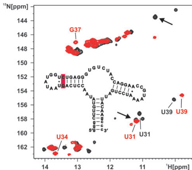
Figure 6. A mutant stabilizing the loop–loop interaction in the free form of the adenine-sensing riboswitch RNA. Overlay of the imino region of a ^1\text{H} , ^{15}\text{N} -HSQC spectrum of the free form of the wild-type adenine-sensing riboswitch RNA (black) and a A30G/U40C double mutant of the adenine-sensing riboswitch RNA (red) both in the absence of \text{Mg}^{2+} . Signals for the imino groups of G37 and U34 are barely visible in the wild-type RNA but are readily detected in the mutant RNA. Only two signals for the uridine imino groups in an U:U base pair are observable in the mutant. In addition, the imino signals for the wobble G:U base pair (arrows) are absent in the mutant. Inset: Secondary structure of the A30G/U40C double mutant. The mutated base pair at the apical tip of helix II is shaded in red.
