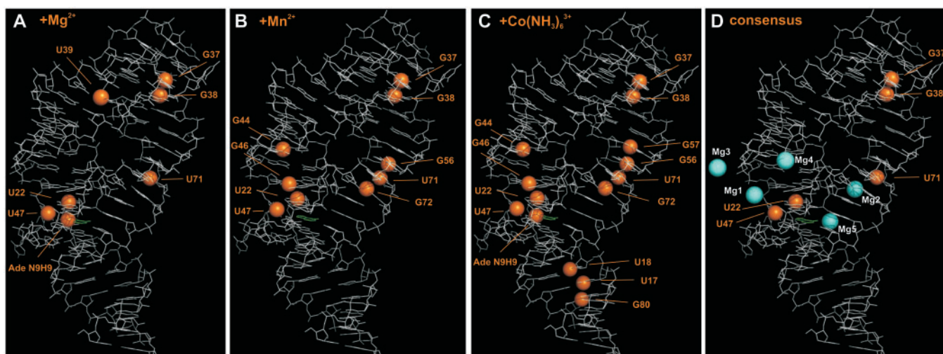
Figure 3. Divalent metal cation-binding sites in solution mapped on the X-ray structure of the closely related add adenine-sensing riboswitch from V. vulnificus in complex with adenine. (A) Imino groups showing chemical shift perturbation upon \text{Mg}^{2+} addition in Figure 2A are represented as orange spheres. There are four regions affected that are located in the ligand-binding core, in the loop-loop interaction, at the apical tip of helix II, and in the center of helix III. (B) Imino groups showing line broadening by paramagnetic \text{Mn}^{2+} in Figure 2B are represented as orange spheres. There are four regions affected that are located in the ligand-binding core, in the loop-loop interaction, and in the center of helix II and helix III. (C) Imino groups showing chemical shift perturbation upon \text{Co}(\text{NH}_3)_6^{3+} addition in Figure 2C and imino groups showing intermolecular NOE contacts to \text{Co}(\text{NH}_3)_6^{3+} in Figure 2D are represented as orange spheres. There are five regions affected that are located in the ligand-binding core, the loop-loop interaction, and in the center of helix I, helix II and helix III. (D) Consensus of imino groups that exhibit all, chemical shift perturbation upon \text{Mg}^{2+} addition, line broadening by paramagnetic \text{Mn}^{2+} , chemical shift perturbation by as well as intermolecular contacts to \text{Co}(\text{NH}_3)_6^{3+} are represented as orange spheres. \text{Mg}^{2+} -ions found in the X-ray structure are shown as cyan spheres and labeled as in (14). \text{Mg}3 is involved in crystal packing. The RNA is drawn in white lines; the adenine ligand is drawn in green lines.
