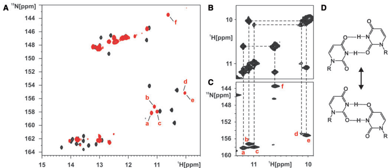
Figure 4. The conformation of the ligand-free adenine-sensing riboswitch RNA in the absence of Mg^{2+} -ions. (A) Overlay of the imino region of a ^1H,^{15}N -HSQC spectrum of the free (red) aptamer domain of the adenine-sensing riboswitch RNA in the absence of Mg^{2+} and in complex with adenine (black). Resonances of the five uridines (a–e) and one guanosine (f) imino groups involved in non-canonical base pairing in the free form of the RNA are labeled with red letters. (B and C) Section of the 2D- ^1H,^1H -NOESY spectrum (B) of the free aptamer domain of the adenine-sensing riboswitch RNA and the corresponding region of the ^1H,^{15}N -HSQC spectrum (C). These spectra show the presence of two different U:U base pairs and one G:U base pair in the free form of the RNA. Imino group correlation in the 2D- ^1H,^1H -NOESY spectrum (B) are indicated by dashed lines and their identity is revealed by dashed lines to the corresponding resonance in the ^1H,^{15}N -HSQC spectrum (C). (D) Two alternative conformations for an asymmetric U:U base pair.
