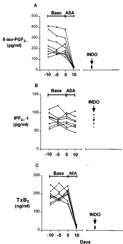
FIG. 4. Serum levels for 8- iso -PGF 2α (A), IPF 2α -I (B), and thromboxane B 2 (C) at 10 and 5 days before aspirin (–10, –5), immediately before aspirin (day 0) (Base), and after 10 days of aspirin intake (ASA). After a 2-week washout, levels were measured after 2-hr indomethacin (INDO) intake.
