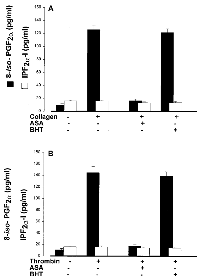
FIG. 5. 8- iso -PGF 2α and IPF 2α -I levels during platelet aggregation induced by collagen (1 μg/ml) (A) or thrombin (0.1 unit/ml) (B). Supernatants were collected before and 3 min after adding the agonist, in the presence of vehicle, aspirin (ASA) (100 μM) or the antioxidant, butylated hydroxytoluene (BHT) (20 μM) ( n = 4 for each panel).
