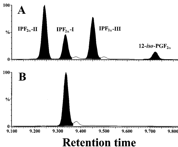
FIG. 2. Specificity of series IPF isolation. (A) A mixture of synthetic IP standards, IPF-I, IPF 2 \alpha -III, and 12- iso -PGF 2 \alpha (a series IV IPF) analyzed by GC/MS. (B) The same mix was added to 100 \mu l of urine and subjected to lactonization, SPE, TLC, saponification, and derivatization as described in the text.
