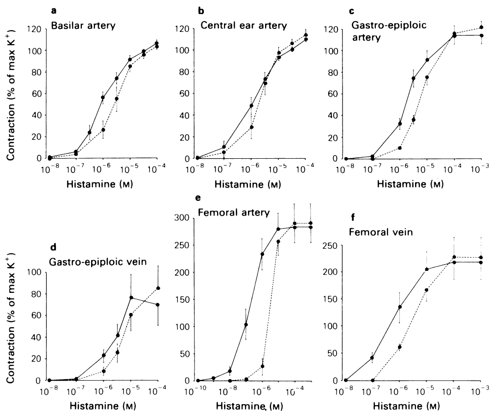
Figure 4 Concentration-response curves for histamine in the absence (interruption line) or presence (continuous line) of 30 nM neuropeptide Y (NPY). (a) Rabbit basilar artery, (b) central ear artery, (c) gastro-epiploic artery, (d) gastro-epiploic vein, (e) femoral artery and (f) femoral vein. The maximum contraction elicited by 137 mM K^+ was set as 100 and the effects of histamine given as a percentage. Means are shown with s.e. means indicated by vertical lines.
