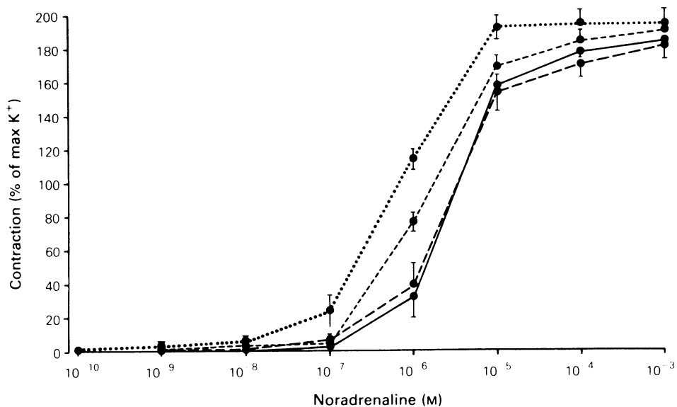
Figure 2 Duration of the potentiation of the response of the rabbit femoral artery to various doses of noradrenaline by 30 nM neuropeptide Y (NPY). NPY was present in the bath for 2 (...), 30 (---) or 60 (---) min before application of noradrenaline (NA). Controls (—) did not receive NPY. Means with s.e.mean, shown by vertical lines. n = 6-8 .
