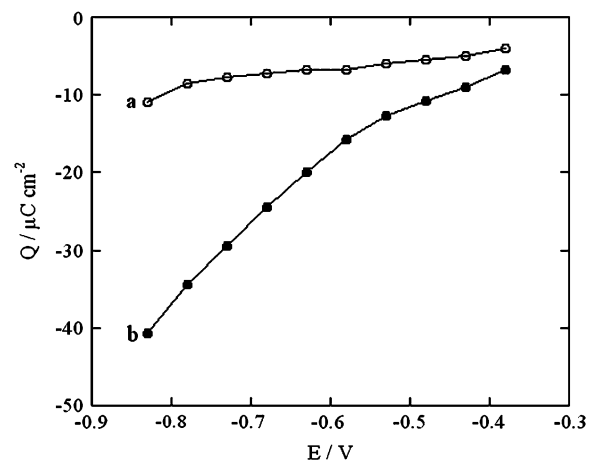
FIGURE 5 Q versus E_f plots at a tBLM incorporating SLN from its 0.7 \mu\text{M} solution in aqueous 0.04 M \text{Na}_2\text{H}_2\text{ATP} before ( a ) and after ( b ) addition of an equal volume of NaCl with the same concentration of \text{Na}^+ ions. Q is the charge recorded upon stepping the potential from a fixed initial value E_i = -0.380 V to progressively more negative values E , after waiting 120 s before each potential jump.
