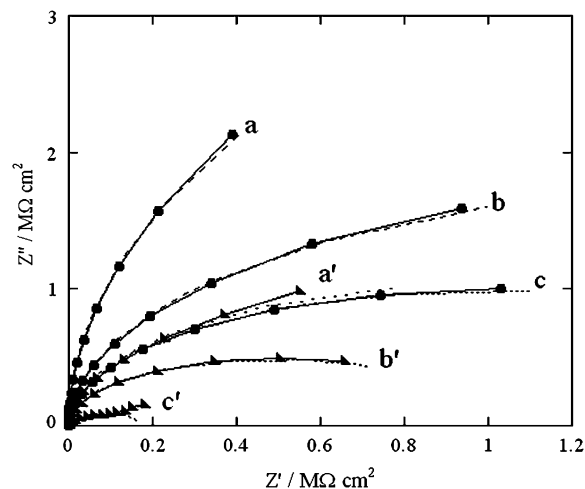
FIGURE 3 Solid curves are Z'' versus Z' plots at a tBLM in 0.1 M KCl at -0.500 V (a), -0.700 V (b), and -0.800 V (c) in the absence of SLN; a', b', and c' are the corresponding plots after incorporation of SLN from its 0.7 \mu\text{M} solution. The dashed curves are fits of the corresponding solid curves to an equivalent circuit consisting of an RC mesh with the solution resistance, R_{\Omega} = 3 \Omega \text{ cm}^2 , in series. The R and C values of the mesh are 11.7 \text{M}\Omega \text{ cm}^2 , 0.73 \mu\text{F cm}^{-2} (a); 2.1 \text{M}\Omega \text{ cm}^2 , 0.77 \mu\text{F cm}^{-2} (a'); 3.6 \text{M}\Omega \text{ cm}^2 , 0.73 \mu\text{F cm}^{-2} (b); 1.0 \text{M}\Omega \text{ cm}^2 , 0.77 \mu\text{F cm}^{-2} (b'); 2.0 \text{M}\Omega \text{ cm}^2 , 0.73 \mu\text{F cm}^{-2} (c); and 0.2 \text{M}\Omega \text{ cm}^2 , 0.90 \mu\text{F cm}^{-2} (c').
