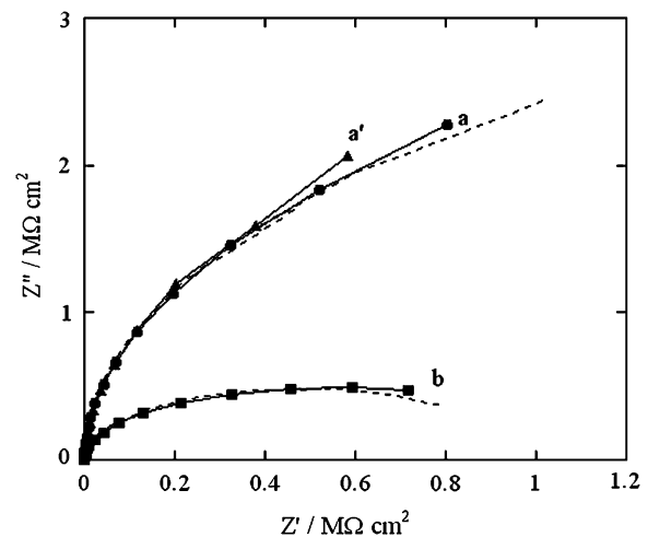
FIGURE 4 Solid curves are Z'' versus Z' plots at a tBLM in a pH 6 aqueous solution of 0.04 M \text{Na}_2\text{H}_2\text{ATP} at -0.580 V in the absence of SLN ( a ), after incorporation of SLN from its 0.7 \mu\text{M} solution ( a' ), and after subsequent dilution with an equal volume of an NaCl solution containing the same concentration of \text{Na}^+ ions ( b ). The dashed curves are fits of the corresponding solid curves to an equivalent circuit consisting of an RC mesh with the solution resistance R_\Omega in series. The R , C , and R_\Omega values of the mesh are 7 \text{ M}\Omega \text{ cm}^2 , 0.56 \mu\text{F cm}^{-2} , 5 \Omega \text{ cm}^2 ( a ), and ( a' ); and 1 \text{ M}\Omega \text{ cm}^2 , 0.57 \mu\text{F cm}^{-2} , 3.5 \Omega \text{ cm}^2 ( b ).
