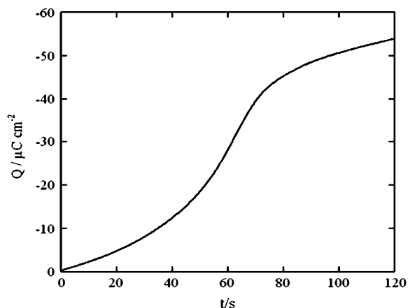
FIGURE 6 Charge versus time curve at a tBLM incorporating SLN from its 0.7 \mu\text{M} solution in aqueous 0.1 M KCl, after a potential jump from -0.300 to -0.800 V.
