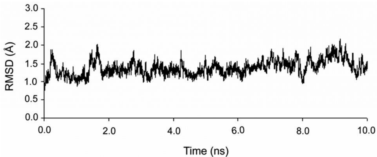
Figure 3. Root-mean-square deviation (RMSD) of the protein backbone and all RNA atoms from the equilibrated structure calculated over the 10 ns simulation of the U1A-SL2 RNA complex.
