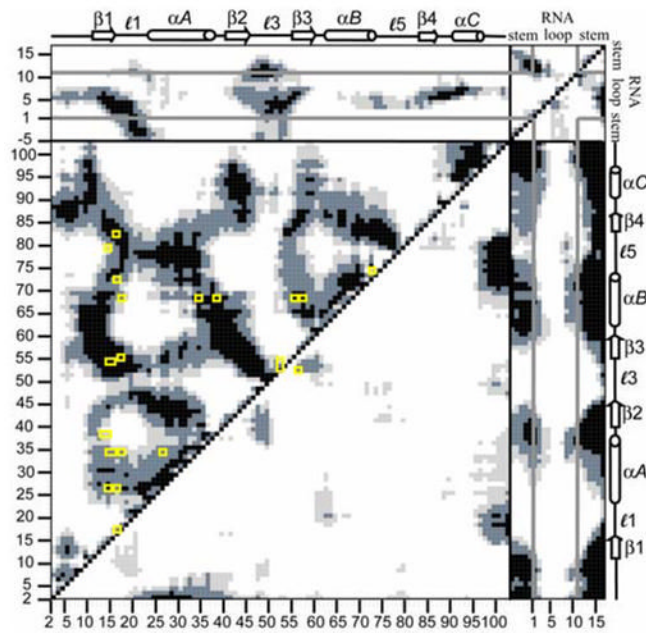
Figure 8. Calculated DCCM for U1A-RNA. Yellow boxes indicate residues revealed to exhibit high covariance from Crowder et al. (2001) statistical covariance analysis of 330 RRM-containing proteins.
