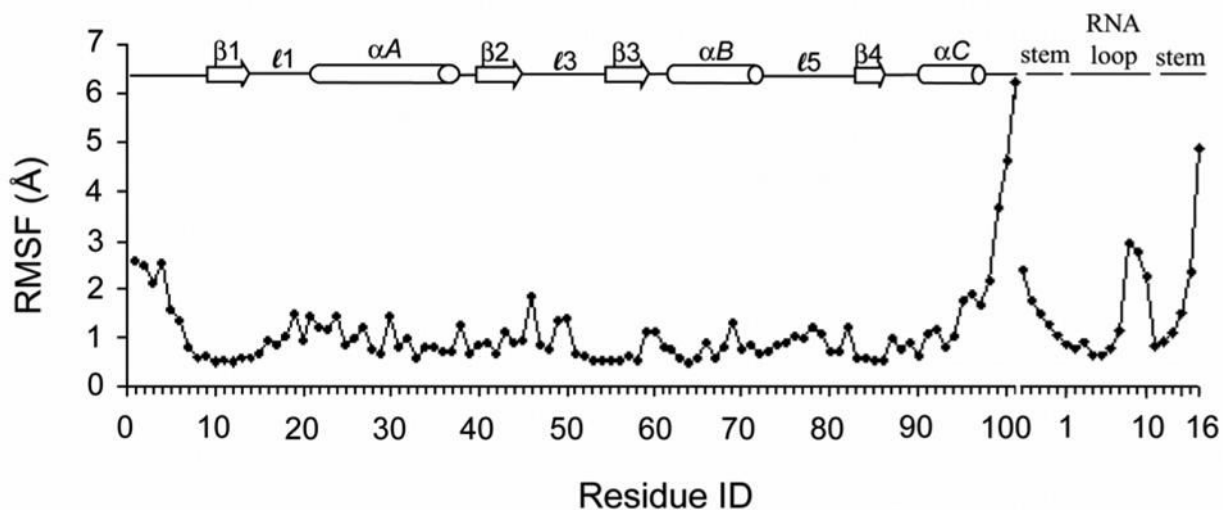
Figure 4. Root-mean-square fluctuations (RMSF) computed on a residue or nucleotide basis with reference to the average structure calculated over the 10 ns simulation of the U1A-SL2 RNA complex.
