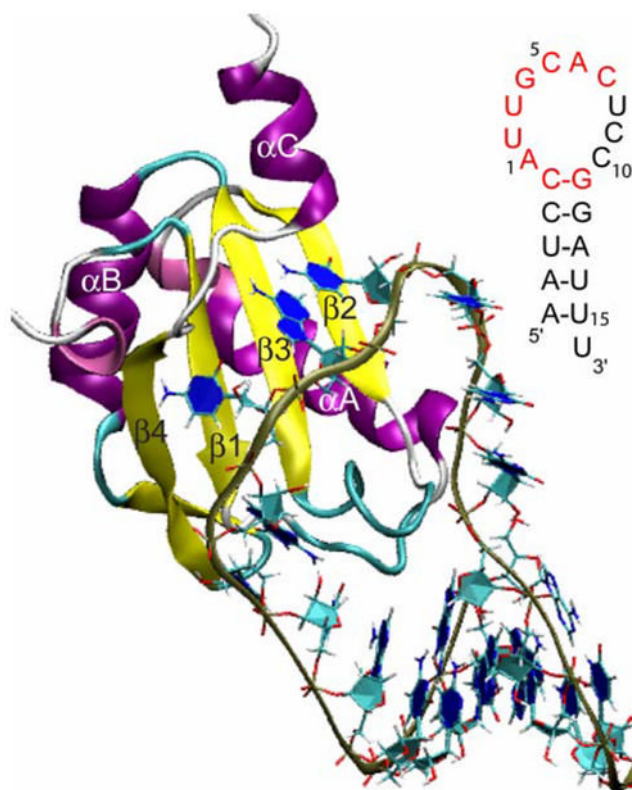
Figure 2. Tertiary structure of the N-terminal RRM of U1A bound to stem-loop 2 RNA (Oubridge et al., 1994). Inset: Nucleic acid sequence of stem-loop 2 RNA with nucleotides recognized by U1A for binding highlighted in red.
