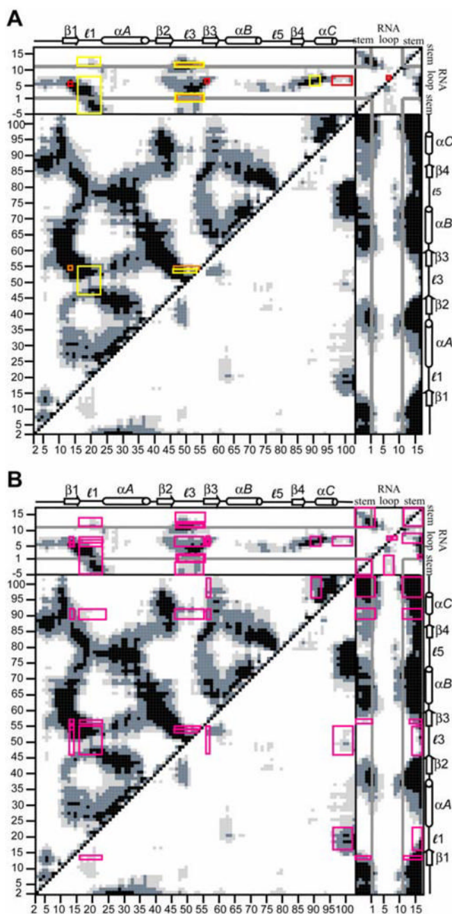
Figure 7. Calculated DCCMs for U1A-RNA indicating residues implicated in cooperativity studies. (A) Red, orange and yellow boxes drawn indicate correlated fluctuations of the residues implicated in networks 1, 2 and 3, respectively. (B) Boxes drawn indicate correlated fluctuations of all residues implicated in the three cooperative networks with each other.
