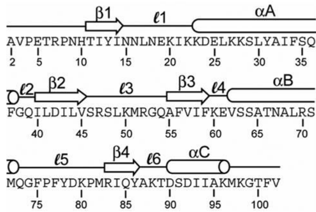
Figure 1. Amino acid sequence of the N-terminal RRM of the protein U1A. Residue numbers are labeled and the secondary structure is indicated above the sequence.
