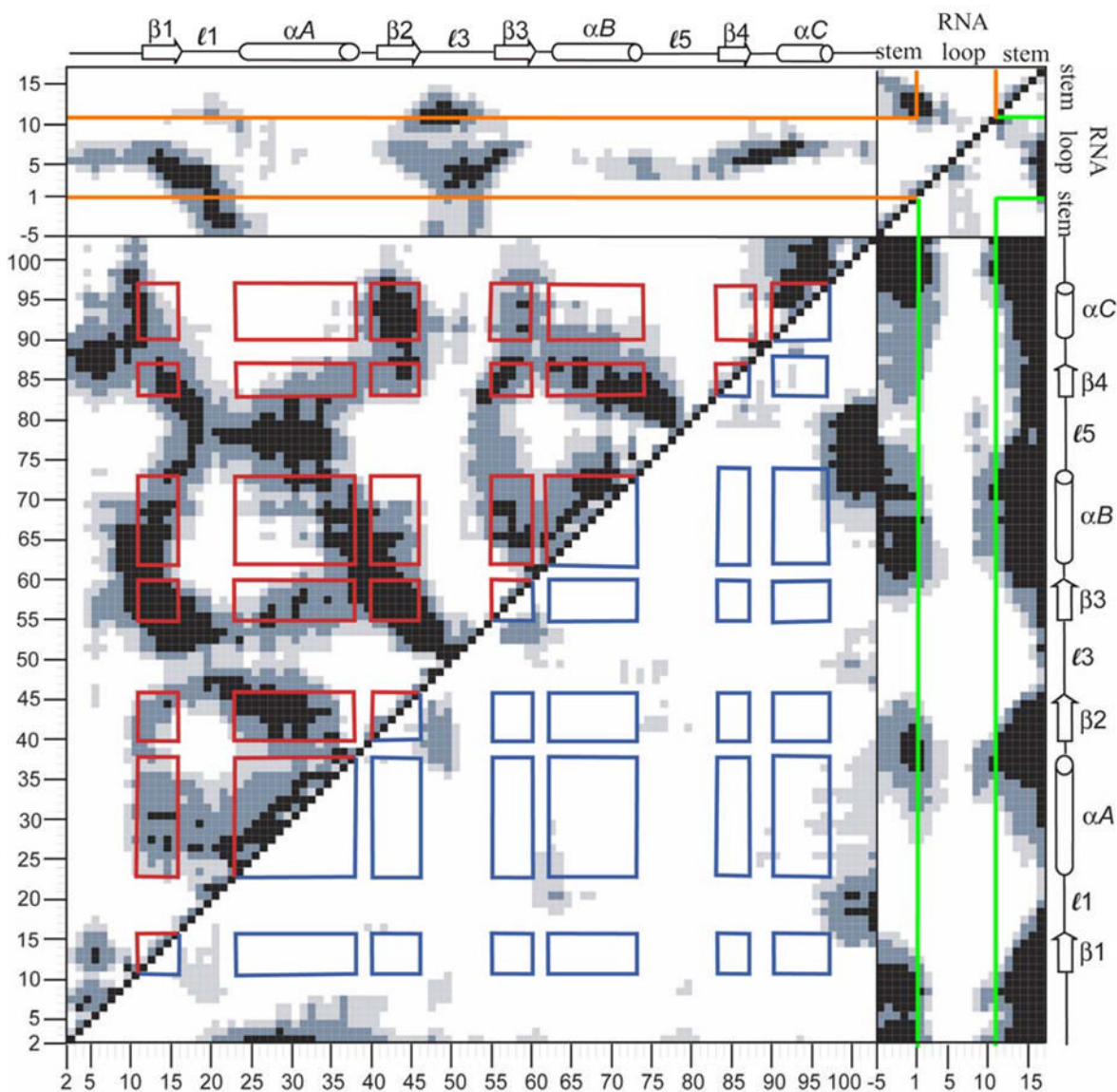
Figure 6. Calculated dynamical cross-correlation map (DCCM) for U1A-RNA. Magnitudes of calculated cross-correlations are indicated via a grey scale with black, slate gray and light gray regions corresponding to strong ( C_{ij} = \pm 0.75-1.00 ), moderate ( C_{ij} = \pm 0.50-0.75 ), and weak ( C_{ij} = \pm 0.25-0.50 ) correlated fluctuations, respectively. Red and blue squares have been drawn to illustrate positive and negative protein-protein secondary structure intersections, respectively. Orange (positive correlations) and green (negative correlations) lines have been drawn to distinguish between RNA stem and loop nucleotides. Additional details can be found in the text.
