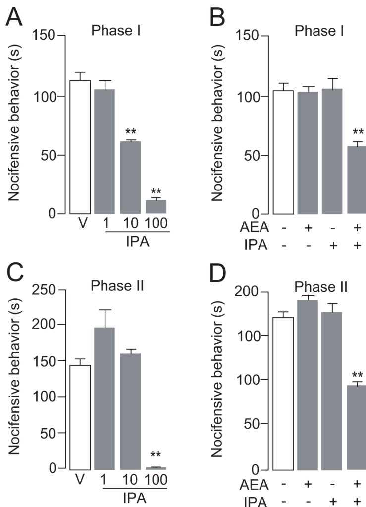
Fig. 2. The BK channel opener isopimaric acid and the endocannabinoid anandamide synergistically inhibit pain behavior. A and C: Dose dependent inhibition of (A) phase I (0-15 min.) or (C) phase II (15-45 min) formalin-evoked pain behavior in Swiss mice by intraplantarly administered isopimaric acid (IPA, 1-100 µg/paw) or vehicle (V). B and D: Effects of anandamide (AEA, 0.1 µg/paw) alone or together with isopimaric acid (IPA, 0.1 µg/paw) on (B) phase I or (D) phase II formalin-evoked pain behavior in Swiss mice (n = 6) ** P < 0.01 vs. V.
