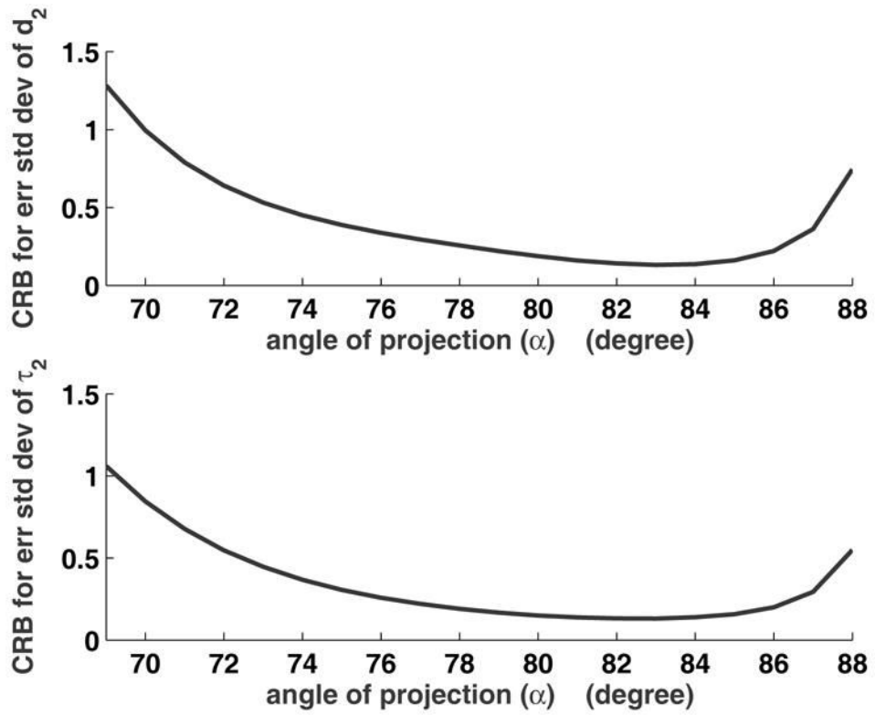
Fig 4. Cramér-Rao bound of the spin density d_2 and half-linewidth \tau_2 versus angle of projection \alpha .
