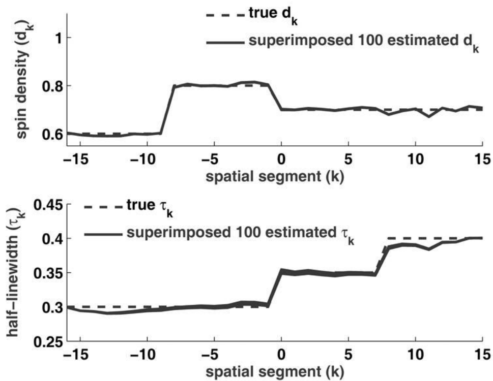
Fig 2. 1D spatial phantom with K = 32 and piece-wise constant spin density and half-lineewidth (dashed lines). Estimated d_k and \tau_k (solid lines) from 100 random initializations and for a fixed noise realization at 30 dB ( \sigma = 0.0051 ). The 100 estimated profiles are superimposed.
