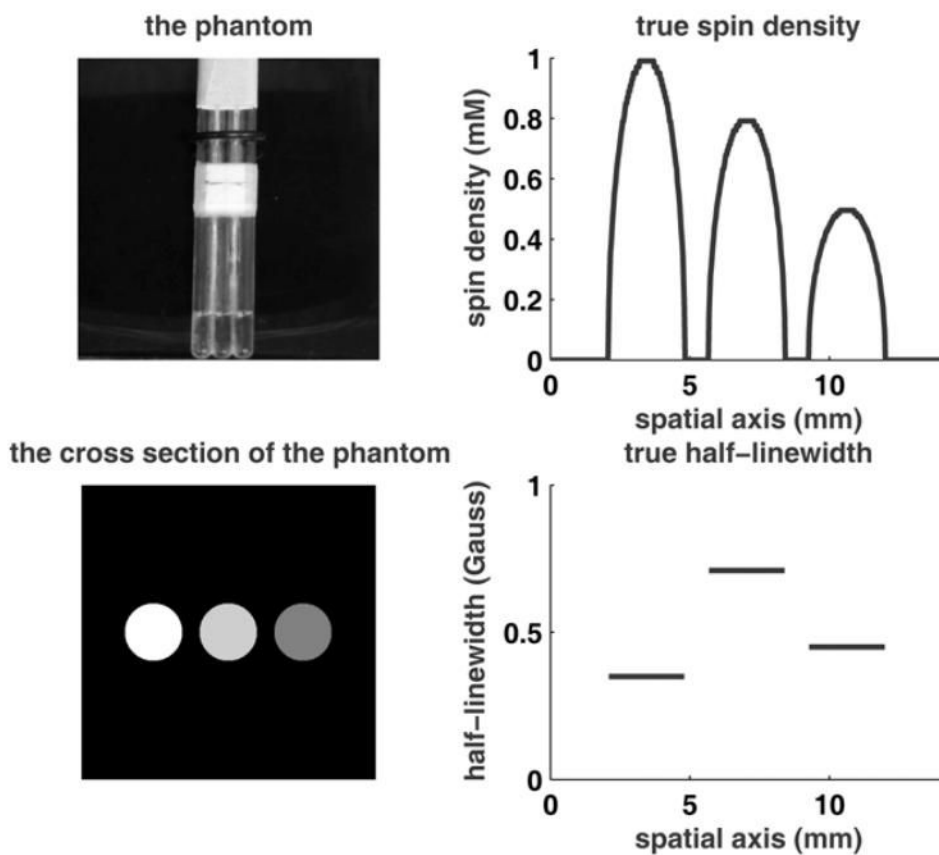
Fig 7. The phantom used for experiment. Top-left: Photograph of the phantom; the three tubes are glued together and filled with nitroxide solutions with three different concentrations mixed with different amounts of the broadening agent. Bottom-left: Schematic of the cross-section of the inner perimeters of the tubes. The magnetic field gradient is along the horizontal axis. Top-right: Spin density profile. Bottom-right: Half-linewidth profile.
