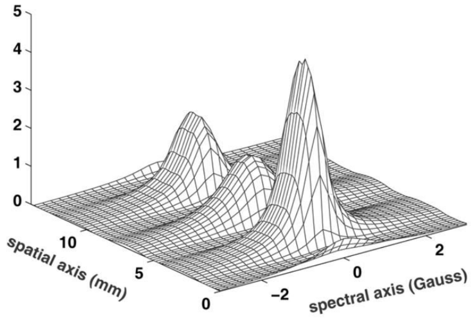
Fig 9. Reconstructed spectral-spatial object from experimental data. Two angles of projections at -83.1^\circ and -69.2^\circ , with 256 samples at each angle, are used. The regularization coefficient is \lambda = 0.01 . The spectral window, \Delta H , is 1.4 G, and the maximum linewidth of the Lorentzian present is 1.4 G.
