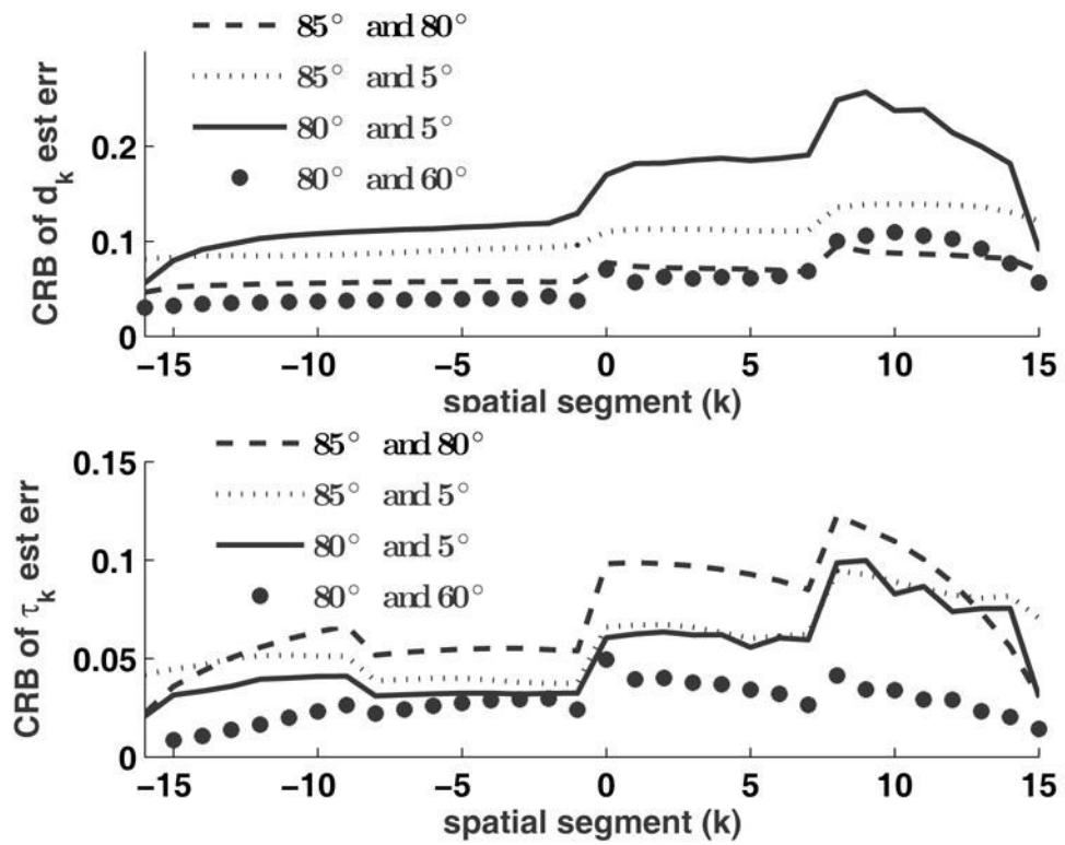
Fig 5. Cramér-Rao bound for the spin density d_k and half-linewidth \tau_k for various combinations of angles of projection \alpha .
