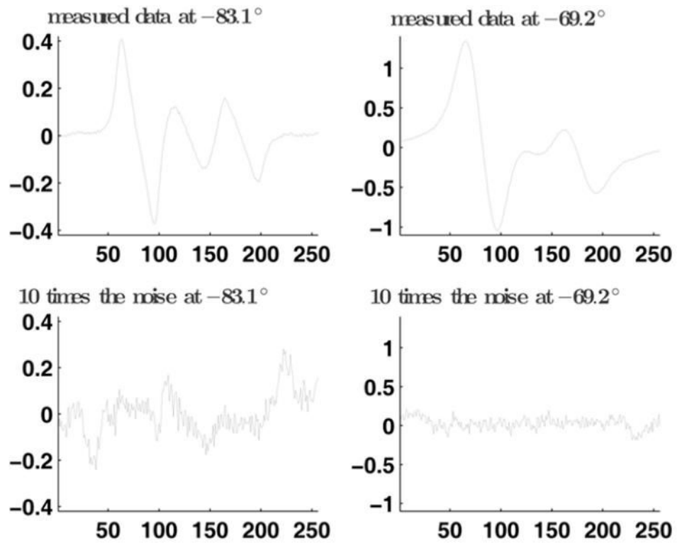
Fig 11. Measured data and residual fit error. Top-left: The measured data at -83.1^\circ . Top-right: Measured data at -69.2^\circ . Bottom-left: 10 times the residual fit error at -83.1^\circ . Bottom-right: 10 times the residual fit error at -69.2^\circ . The vertical axis is in arbitrary unit and the horizontal axis denotes sample number.
