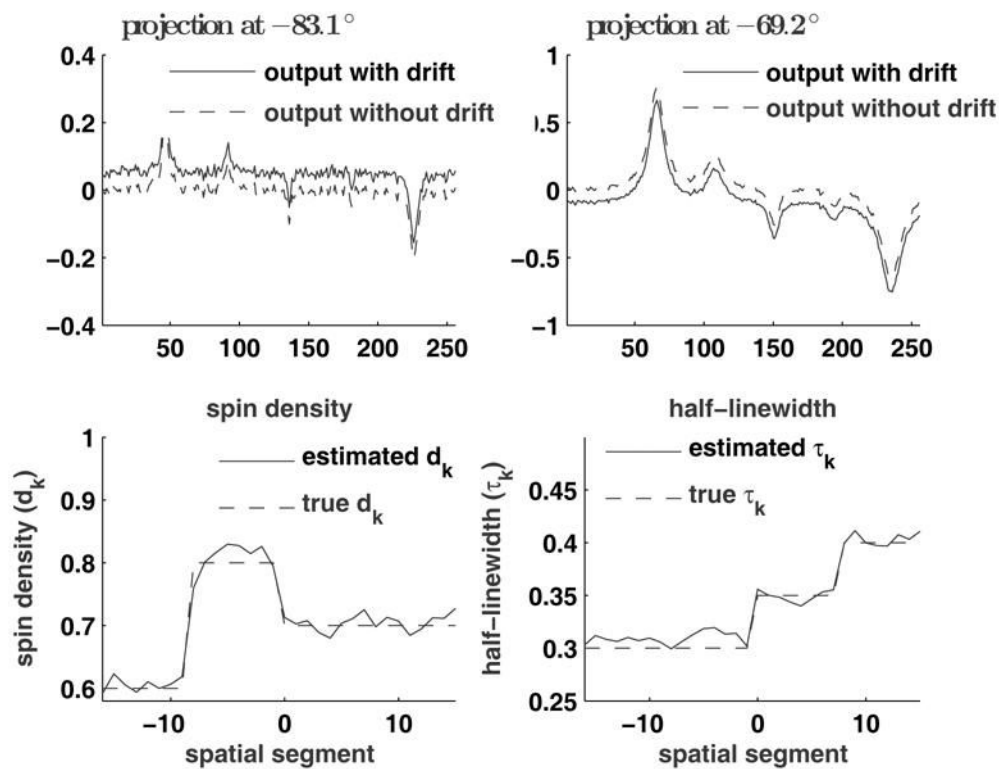
Fig 6. Projections with and without baseline drift and true and estimated parameters. The data with baseline drift were used for parameter estimation. A linear baseline correction model on the unmodulated projection was assumed and the same correction model gives a constant drift correction in the modulated projection model. At the -83.1^\circ projection the drift is positive and at -69.2^\circ projection the drift is negative. The SNR value is 25 dB and the regularization constant \lambda = 0.1 .
