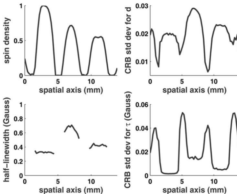
Fig 10. Top-left: Reconstructed spin density ( d_k ) values from experimental data. Bottom-left: Reconstructed half-linewidth ( \tau_k ) values. Top-right: Cramér-Rao bounds for estimation error standard deviations of d_k . Bottom-right: Cramér-Rao bounds for estimation error standard deviations of \tau_k . The d_k and \tau_k estimates are accepted if the CRB is less than 10 times the minimum of CRB across all k , otherwise they are discarded and not shown in the left column d_k and \tau_k plots.
