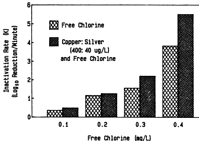
FIG. 2. Inactivation of L. pneumophila by exposure to electrolytically generated copper and silver (400 and 40 µg/liter) and/or various concentrations of free chlorine.
