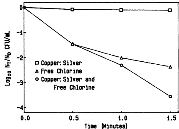
FIG. 4. Reduction of L. pneumophila by exposure to electrolytically generated copper and silver (400 and 40 µg/liter) and/or free chlorine (0.4 mg/liter).
