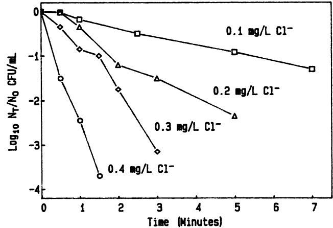
FIG. 3. Reduction of L. pneumophila by exposure to electrolytically generated copper and silver (400 and 40 µg/liter) and various concentrations of free chlorine.
