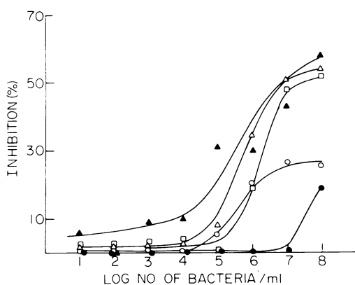
FIG. 2. Effects of different blocking treatments in competition ELISA. The treatments used were no blocking (●), 1% egg albumin (▲), 1% bovine serum albumin (○), 1% ethanolamine (□), and 10^9 CFU of isolate 1023 or X. campestris pv. vesicatoria per ml (△). Experimental conditions were as described for Fig. 1e. Data are presented without preincubation of antibody and bacteria.
