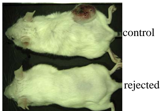
Figure 5 Long-term anti-tumor immunity. Mice that rejected the initial i.d. tumor derived from CT-26 cells were re-challenged intradermally with 5 \times 10^6 parental cells 8 months after the initial tumor eradication (9 months after the initial tumor inoculation). Tumor growth was observed after 30 days (upper: a control mouse; lower: a mouse that previously eradicated the initial tumor). n = 2.
