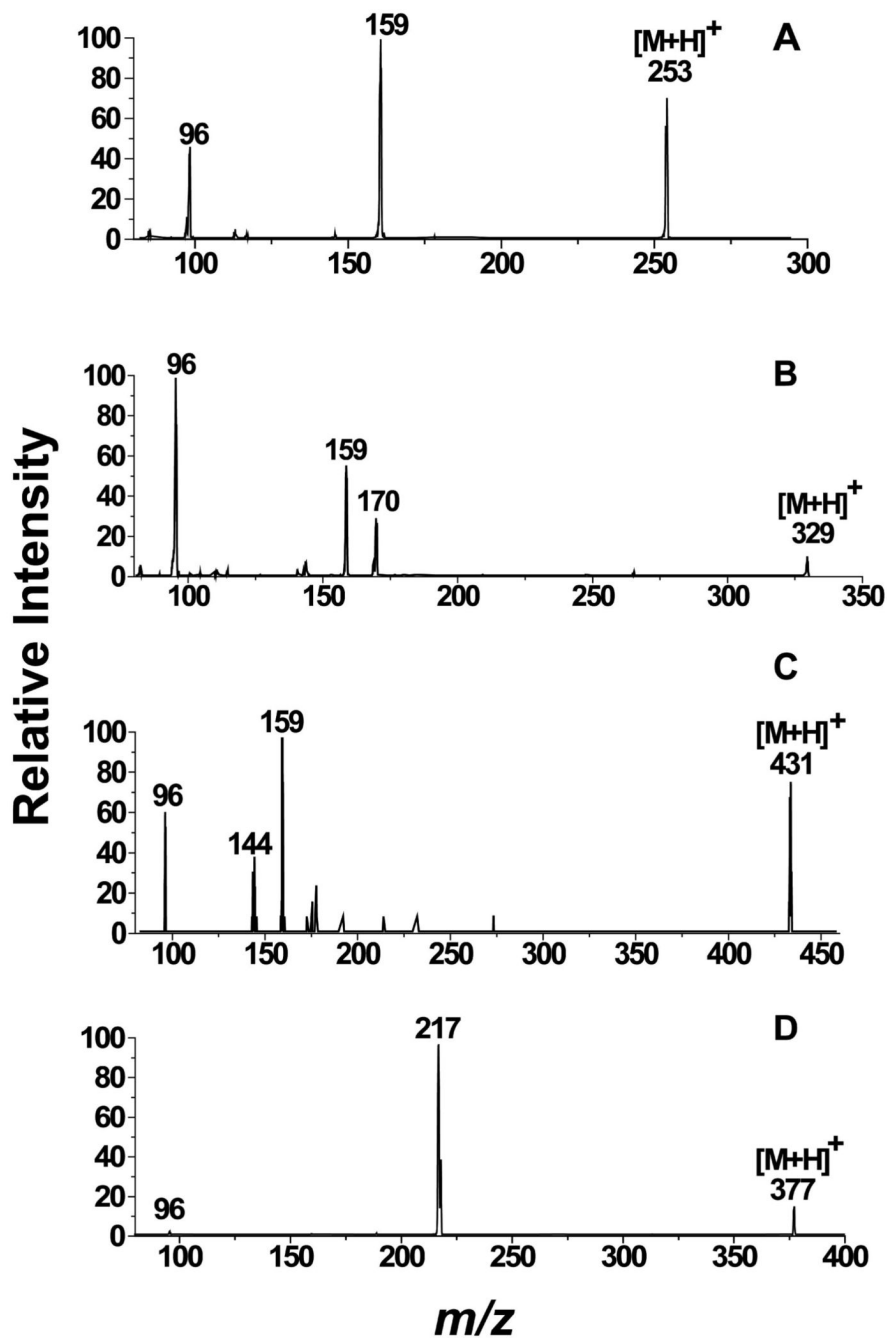
Fig 2. LC-ESI-MS/MS product ion spectra of the [M+H]^+ ions of DMIS derivatives. Shown are product ion spectra of (A) DMIS-phenol at 25 eV collision energy; (B) DMIS-phenylphenol at 30 eV collision energy; (C) DMIS- E_2 at 40 eV energy; and (D) DMIS-1-hydroxypyrene at 25 eV collision energy.
