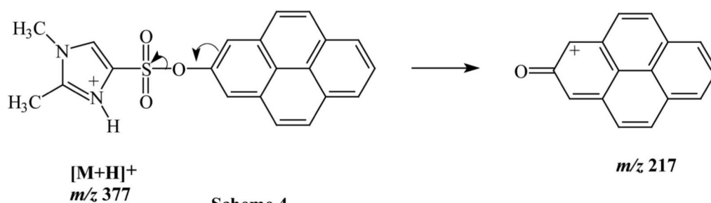
Fig 3. Proposed fragmentation pathways for CID of the DMIS derivatives of phenolic compounds based on LC-ESI-MS/MS product ion spectra. Schemes 1 through 3 are proposed for the formation of ions of m/z 159, 96, and 144 from the dimethylimidazole moieties of the protonated DMIS derivatives of phenolic compounds that are commonly observed in the product ion spectra. Scheme 4 is proposed for the formation of a highly resonance-stabilized ion derived from the 1-hydroxypyrene moiety after heterolytic cleavage of the protonated 1-hydroxypyrene DMIS derivative.
