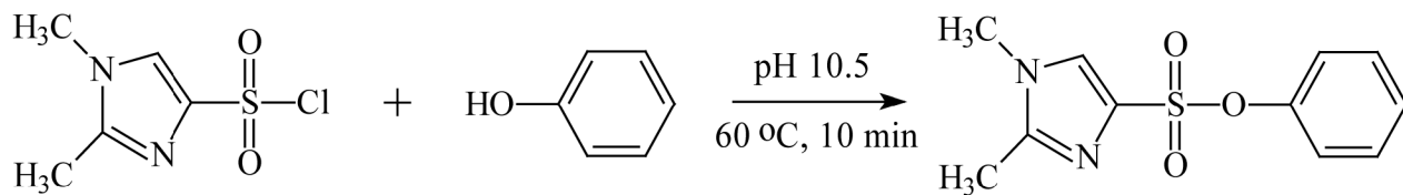
Fig 1. Derivatization of phenol by reaction with DMISC.
