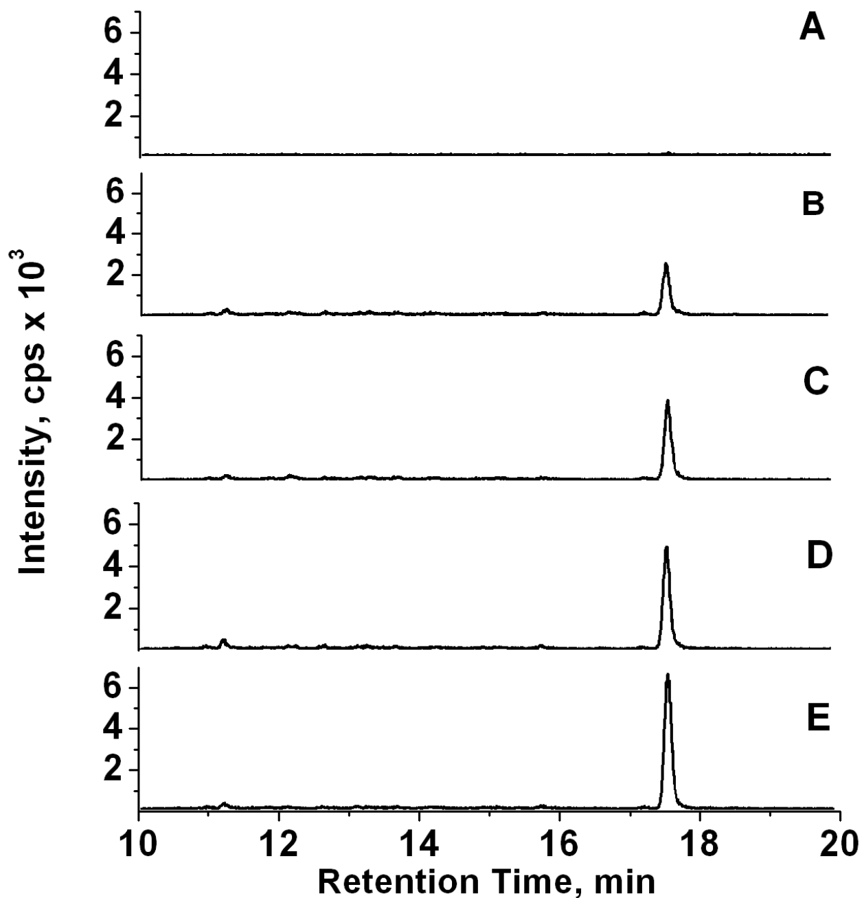
Fig 5. LC-ESI-MS/MS analysis of urinary 1-hydroxypyrene as its DMIS derivative. Samples (1 mL) were processed as described in the Experimental section. Shown are selected reaction ion chromatograms from the analysis of 1-hydroxypyrene as its DMIS derivative, monitoring the positive ion MS/MS transition of m/z 377 \rightarrow 217, in (A) artificial urine as the blank, (B) the unspiked human urine pool, and the urine pool spiked with (C) 50 pg, (D) 100 pg, and (E) 200 pg of 1-hydroxypyrene.
