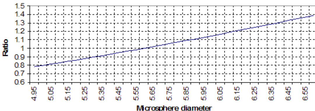
Figure 5 Graph of the ratio of fluorescent intensity to true normal by bead size. A ratio of 1 is for a microsphere sample equal to the specified mean microsphere diameter. This shows the relationship of microsphere diameter to brightness of signal, illustrating the correspondence of brightness as an r^2 relation.
