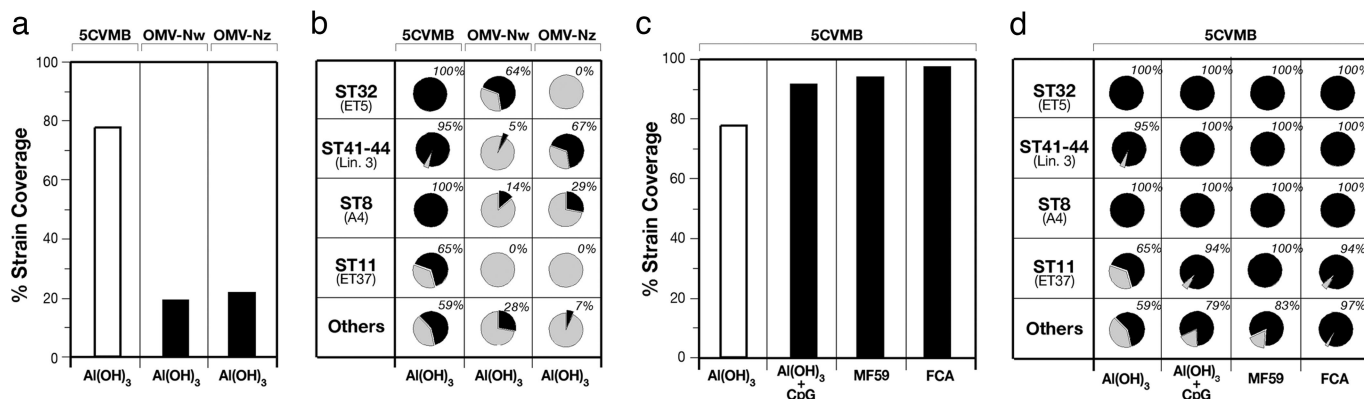
Fig. 3. Protective effect of 5CVMB vaccine. The analysis has been performed by testing the immune sera for BCA against 85 N. meningitidis strains using baby rabbit serum as complement source (16). Results are expressed as the percentage of strains killed with titers \geq 128 . (a and b) Comparison of strain coverage induced by 5CVMB, OMV-Nw, and OMV-Nz vaccines (a) and the respective vaccine coverage of the 85 strains grouped into hypervirulent clusters (b). (c and d) Strain coverage induced by different formulations of 5CVMB vaccine (with aluminum hydroxide, aluminum hydroxide plus CpG 1826, MF59, or FCA) (c) and the respective vaccine coverage of hypervirulent clusters (d).
