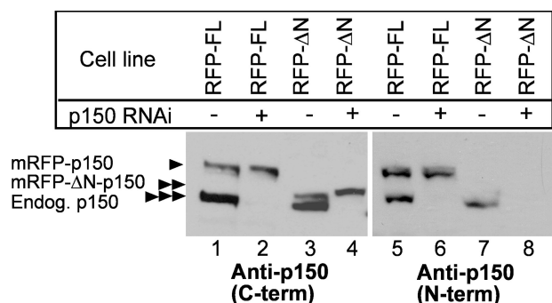
Figure 1. Western blots of extracts of S2 cells expressing mRFP-p150 glued or mRFP- \Delta N-p150 glued . mRFP-p150 glued , lanes 1, 2, 5, and 6; mRFP- \Delta N-p150 glued , lanes 3, 4, 7, and 8. Endogenous p150 glued was depleted by using RNAi against the 3' UTR of p150 glued mRNA (lanes 2, 4, 6, and 8). Lanes 1–4 were probed with an antibody against the C-terminal fragment of p150 glued ; lanes 5–8 were probed with an antibody against the N-terminal fragment of p150 glued . Positions of mRFP-p150 glued , mRFP- \Delta N-p150 glued , and endogenous p150 glued bands are marked by single, double, and triple arrowheads, respectively.
