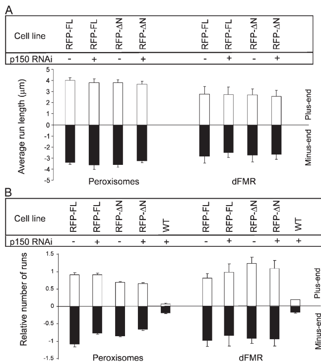
Figure 6. Deletion of the microtubule-binding domain of p150 glued has no effect on the mean run length or relative number of runs of both peroxisomes and dFMRP particles. (A) Mean run length; (B) relative number of runs. Note that the relative number of runs in cells having no p150 glued expression dropped more than fivefold compared with the cells expressing mRFP-p150 glued or mRFP-ΔN-p150 glued . The mean run length is calculated from the trajectory length of moving particles in the process without stopping or changing directions. The total number of particles analyzed for each treatment group in this experiment was 83, 147, 256, 268, and 113 for peroxisomes and 172, 142, 170, 337, and 111 for dFMR (numbers correspond to bars on the chart from left to right). Error bars represent SD.
