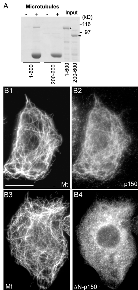
Figure 3. Truncation of the first 200 amino acid residues of p150 glued eliminates microtubule binding. (A) Recombinant proteins purified and incubated with taxol-stabilized microtubules are centrifuged to pellet with microtubules. Pellets were analyzed by SDS-gel electrophoresis. Inputs are proteins used for the assay, and asterisks mark positions of His 6 -p150 glued (residues 1–600) or His 6 -p150 glued (residues 200–600). (B) EGFP-tagged p150 glued (B2) is aligned along microtubules (B1), and EGFP-ΔN-p150 glued (B4) shows no microtubule binding. Cells were treated with 3' UTR RNAi to deplete endogenous p150 glued , extracted with detergent, and stained with a monoclonal antibody against α-tubulin and EGFP polyclonal antibody. Bar, 10 μm.
