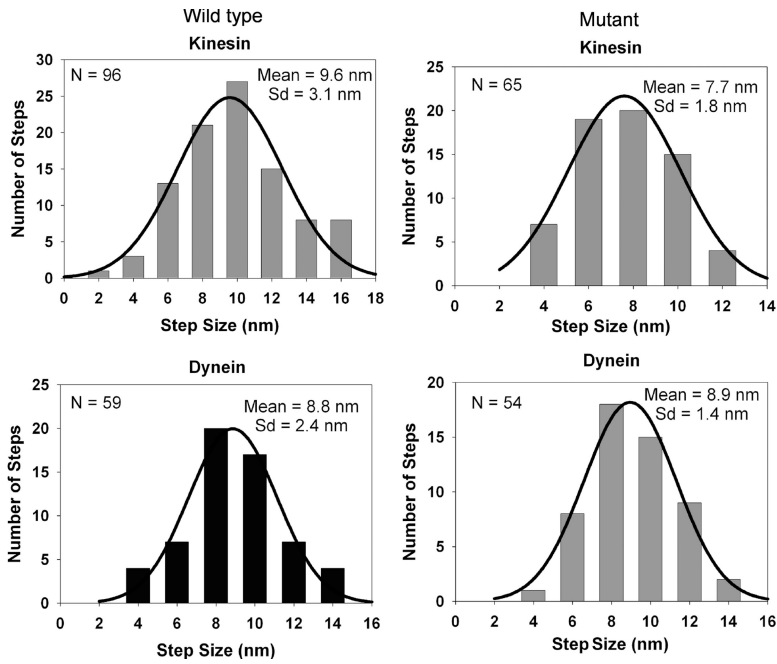
Figure 7. Step sizes of cytoplasmic dynein- or kinesin-transporting peroxisomes are not altered by truncation of the microtubule-binding domain of p150 glued . Histograms of the distribution of the individual steps of kinesin and dynein show that the mean step sizes are ~8 nm in both wild-type (mRFP-p150 glued ) and mutant (mRFP-ΔN-p150 glued ) cells.
