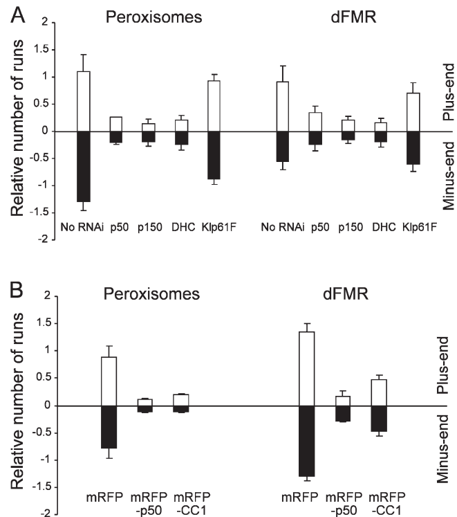
Figure 5. Dynactin and dynein are required for the bidirectional movement of peroxisomes and dFMRP particles. (A) The relative number of runs (see Materials and methods) of both peroxisomes and dFMRP particles dramatically dropped after the knockdown of dynein subunits (p50 or p150 glued ) or DHC. RNAi against the mitotic kinesin Klp61F was used as a control. (B) The relative number of runs of both peroxisomes and dFMRP particles substantially dropped after the overexpression of dominant-negative inhibitors of dynein, mRFP-p50, or mRFP-tagged coiled-coil 1 of p150 glued (mRFP-CC1). Error bars represent SD.
