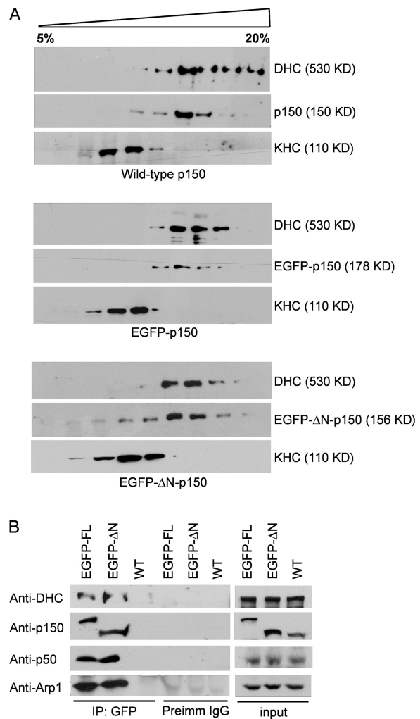
Figure 2. The truncated form of p150 glued and ΔN-p150 glued forms the dynein complex and interacts with cytoplasmic dynein. (A) Sucrose gradient fractionation of extracts from S2 cells expressing wild-type p150 glued , EGFP-p150 glued , or EGFP-ΔN-p150 glued . EGFP-ΔN-p150 glued sediments at the same rate as wild-type p150 glued or EGFP-p150 glued . KHC is used as a control, which sediments differently from dynein and dyneactin. (B) Extracts from cells expressing EGFP-p150 glued or EGFP-ΔN-p150 glued and untransfected cells were immunoprecipitated with an anti-EGFP antibody or control preimmune IgG. Precipitates were probed using anti-DHC antibody and antibodies against dyneactin subunits p150 glued , p50, and Arp-1. Note that EGFP antibody but not the control IgG pulls down cytoplasmic dynein and dyneactin subunits. Inputs are cell extracts from each sample.
