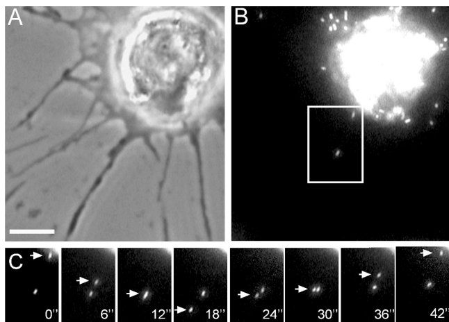
Figure 4. Morphology and peroxisome distribution in S2 cells spread on the substrate in the presence of cytochalasin D. (A and B) Phase-contrast (A) and fluorescent (B) images of an S2 cell expressing EGFP-tagged peroxisomes in the presence of cytochalasin D. (C) Frames from a time-lapse video [Video 4, available at http://www.jcb.org/cgi/content/full/jcb.200608128/DC1 ] show bidirectional movements of peroxisomes. Frames correspond to the boxed area in B. Time in seconds is indicated on each frame. Arrows show a peroxisome moving in the process. Bar, 5 \mu m.
