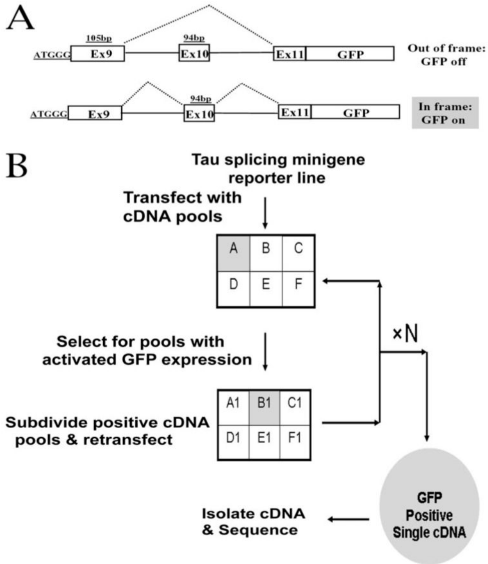
FIGURE 1. A , a schematic diagram of the Tau4R-GFP reporter constructs. The tau splicing reporter gene is designed in such a way that GFP is only expressed when the exon 10 is included (for a detailed description of the reporter gene construction, see "Experimental Procedures"). B , a diagrammatic representation of the cDNA library screening protocol based on GFP expression following progressive division and subdivision of cDNA pools and transfection of cDNA pools into the stable cell line expressing Tau4R-GFP reporter.
