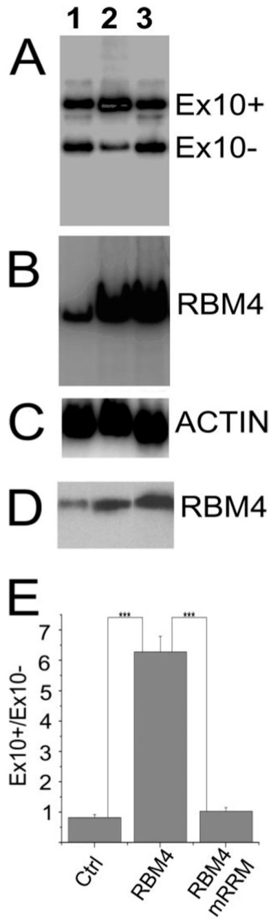
FIGURE 4. The RNA recognition domain of RBM4 is essential for its activation of tau exon 10 inclusion
