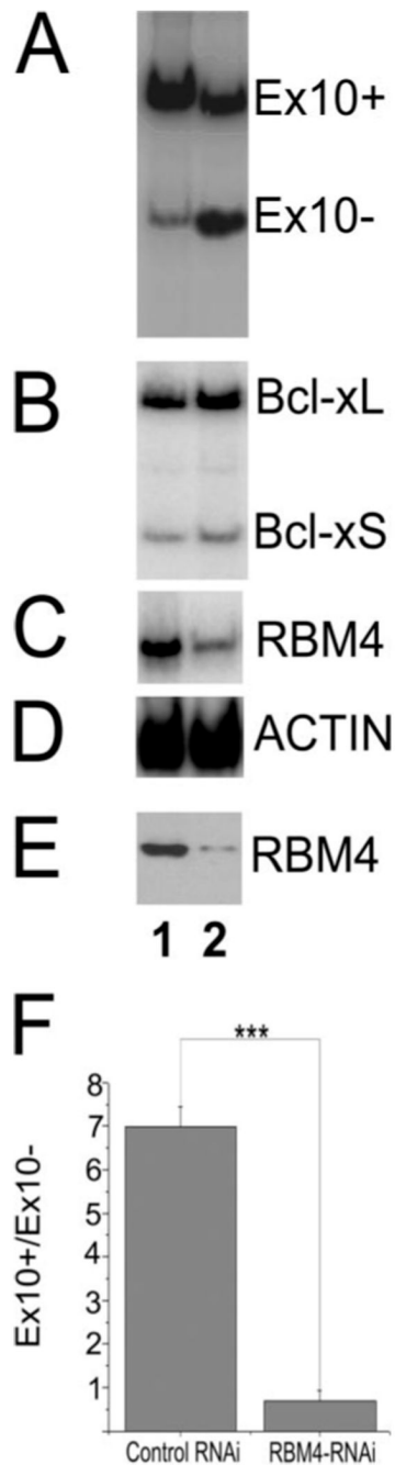
FIGURE 7. RNAi-mediated knockdown of RBM4 decreases tau exon 10 inclusion RNAi specific for human RBM4 ( lane 2 ) or control RNAi ( lane 1 ) was co-transfected with Tau minigene TauEx9-10-11 (wild type) into HEK293 cells as described under "Experimental Procedures." RNA preparations or protein lysates were made 48 h post-transfection and analyzed by RT-PCR or Western blotting. A , tau exon 10 alternative splicing isoforms as detected by RT-PCR. B , the alternative splicing pattern of Bcl-x detected by RT-PCR using Bcl-x-specific primers. C , the level of RBM4 RNA detected by RT-PCR. D , the level of actin transcript as detected by RT-PCR as the internal control. E , the levels of RBM4 protein expression detected by Western blotting using specific anti-RBM4 antibody. F , the quantification of tau Ex10 splicing isoforms as shown in A . The results are derived from six
