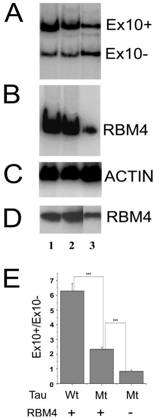
FIGURE 6. Mutation in the RBM4 putative binding site in tau pre-mRNA affects the exon 10 splicing stimulatory activity of RBM4
