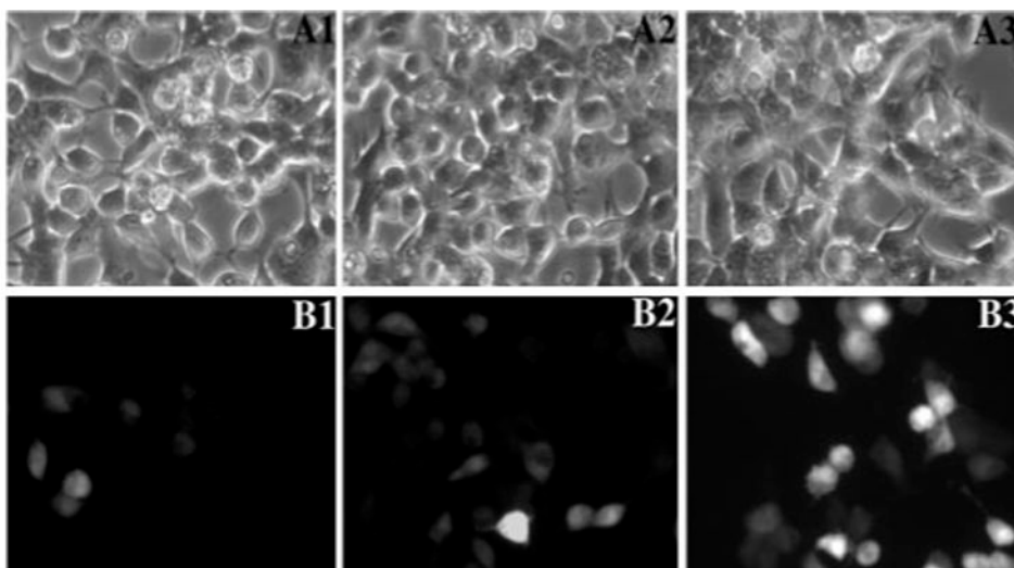
FIGURE 2. The expression of Tau-GFP reporter during the cDNA library screening The stable HEK293 cell line expressing the Tau4R-GFP reporter gene was used for screening cDNA library. A progressive subdividing-retransfecting method was used to identify cDNAs encoding potential regulators of tau alternative splicing, as described under "Experimental Procedures." GFP fluorescence was monitored by fluorescent microscopy following the transfection of pools of cDNAs prepared from the cDNA library. A1–A3 , phase-contrast images; B1–B3 , corresponding fluorescent microscopic images. These experiments show progressive enrichment of GFP-expressing cells following the primary round ( B1 ), the third round ( B2 ), and the sixth round ( B3 ) of subdivision and retransfection of the positive cDNA pools.
