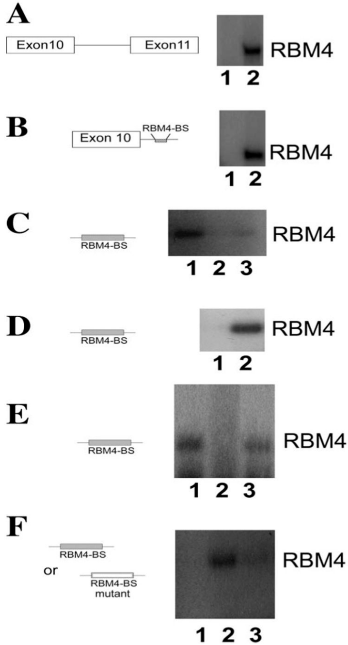
FIGURE 5. RBM4 interacts with an intronic element downstream of the 5' splice site of exon 10 in tau pre-mRNA
