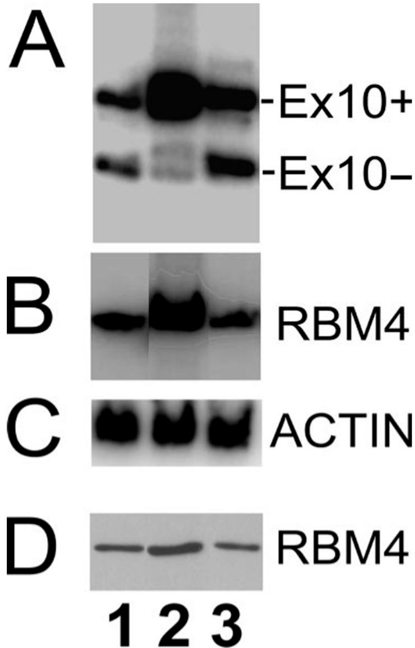
FIGURE 3. Overexpression of RBM4 protein increases the inclusion of tau exon 10 in transfected cells
