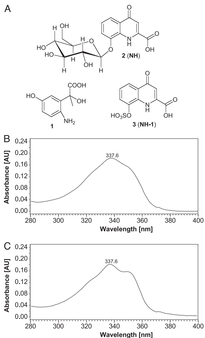
Fig. 3. Chemical properties of identified compounds. (A) Structures of 1, 2 (NH), and 3 (NH-1). (B) The 280- to 400-nm region of the UV spectrum of NH. (C) UV spectrum of NH-1.
