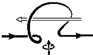
FIG. 1. A flux rope twisted into an \Omega by a right-handed motion. The loop is accompanied by an electric current antiparallel to the magnetic field (14).
