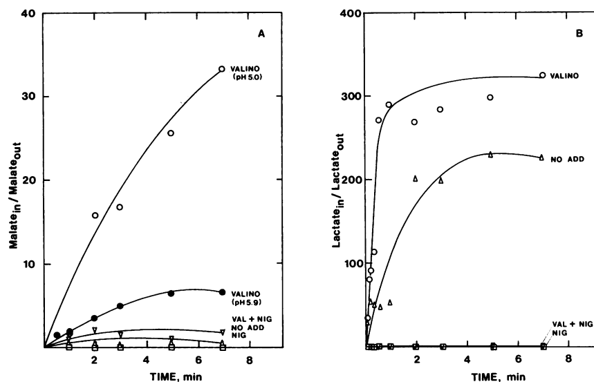
FIG. 8. Uptake of L-malate (A) and L-lactate (B) in membrane vesicles of L. lactis IL1441-SO1 fused with cytochrome c oxidase-containing liposomes. L-[ 14 C]malate (20 \mu M, final concentration) and L-[ 14 C]lactate (2.8 \mu M, final concentration) uptake by the fused membranes was assayed in KPi/KCl buffer, pH 5.0 (open symbols) and pH 5.9 (closed symbols), at 25°C and at final protein concentrations of 0.23 and 0.11 mg/ml for L-malate and L-lactate uptake, respectively. The electron donor system, potassium ascorbate-TMPD-cytochrome c, was present in all samples. Valinomycin (valino, val) and nigericin (nig) were added to final concentrations of 0.6 and 0.3 \mu M, respectively. No add, no addition.
