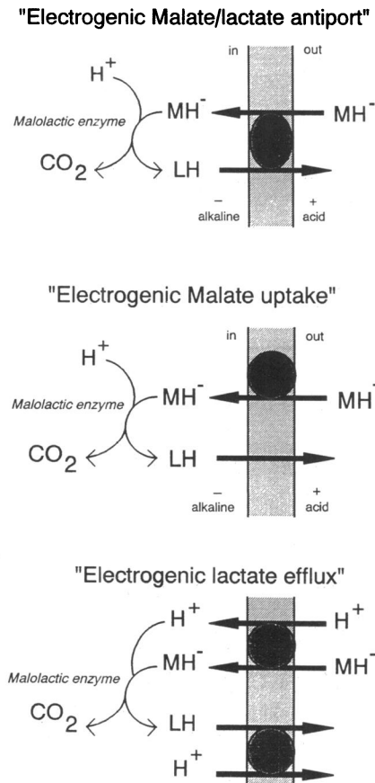
FIG. 1. Possible mechanisms for the generation of metabolic energy by malolactic fermentation based on electrogenic malate/lactate antiport, electrogenic malate uptake, and electrogenic lactate efflux. MH^- , monoanionic L-malate; LH, L-lactic acid.
