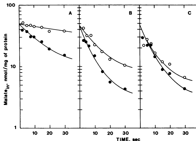
FIG. 7. Effect of membrane potential on efflux and exchange of L-malate in membrane vesicles of L. lactis IL1441-SO1 fused with liposomes. Fused membranes were loaded with 6.5 mM potassium-L- ^{14}\text{C} malate in KPi/KCl buffer, pH 5.0, in the presence of valinomycin (2 nmol/mg of protein) as described in Materials and Methods. L- ^{14}\text{C} malate efflux (A), heterologous L- ^{14}\text{C} malate/L-lactate exchange (B), and homologous L- ^{14}\text{C} malate/L-malate exchange (C) were assayed at 25°C upon 80-fold dilution of the membranes into KPi/KCl buffer, pH 5.0 (open circles), or 50 mM sodium phosphate-100 mM NaCl-2 mM \text{MgSO}_4 , pH 5.0 (closed circles). L-Lactate (B) and L-malate (C) were present as potassium (open circles) or sodium (closed circles) salts at final concentrations of 5 mM. The final protein concentration in the assay mixture was 0.15 mg/ml.
