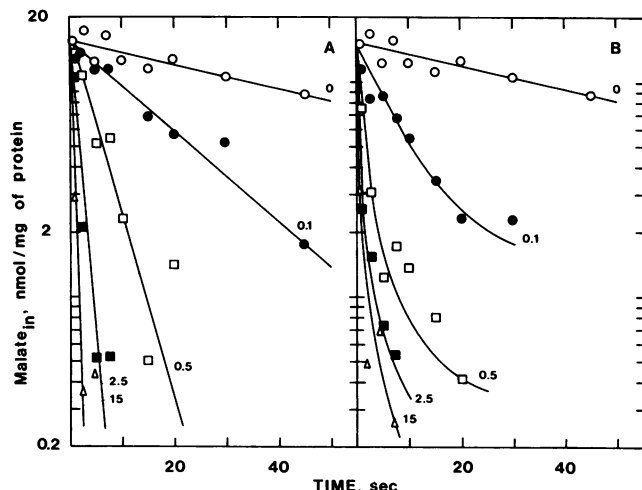
FIG. 6. Efflux and exchange of L-malate in membrane vesicles of L. lactis IL1441-SO1. Membrane vesicles were loaded with 5 mM potassium-L- ^{14}\text{C} malate in KPi/KCl buffer, pH 5.9, as described in Materials and Methods. Efflux (open circles) and exchange (other symbols) were assayed at 25°C upon 80-fold dilution of the membrane vesicles into KPi/KCl buffer containing various concentrations of potassium-L-lactate (A) and potassium-L-malate (B) (concentrations [millimolar] are indicated). The final protein concentration in the assay mixture was 0.39 mg/ml.
