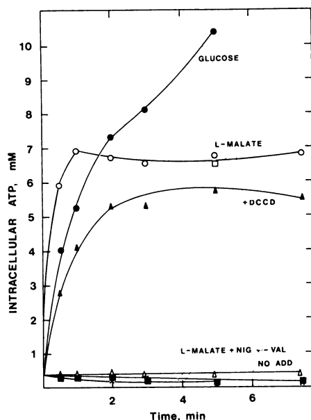
FIG. 3. Intracellular ATP concentrations. L-Lactate (100 mM)-loaded L. lactis IL1403 cells were diluted 100-fold into 50 mM K-MES plus 2 mM MgSO_4 , pH 5.0, containing 20 mM potassium-L-malate or 10 mM glucose. At the times indicated, samples were withdrawn and analyzed for ATP content. Valinomycin (val) and nigericin (nig) concentrations were 2 and 1 \mu M , respectively. DCCD, cells treated with 100 \mu M DCCD for 1 h at 30°C; no add, no exogenous energy source present. The experiments were carried out at 30°C.
