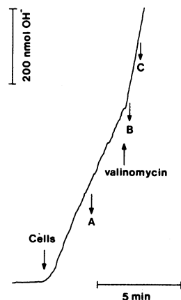
FIG. 4. Measurement of malolactic fermentation activity. At the times indicated, 10 \mu l of L-lactate (50 mM)-loaded L. lactis IL1403 cells (33.2 mg of protein per ml) were diluted into 4 ml of K-MES/KCl buffer, pH 5.0, containing 5 mM potassium-L-malate. The pH trace indicates the alkalization of the medium. Arrows indicate the addition of cells and valinomycin (1 \mu M , final concentration); A, B, and C indicate when samples were withdrawn for the determination of L-lactate (see Table 1).
